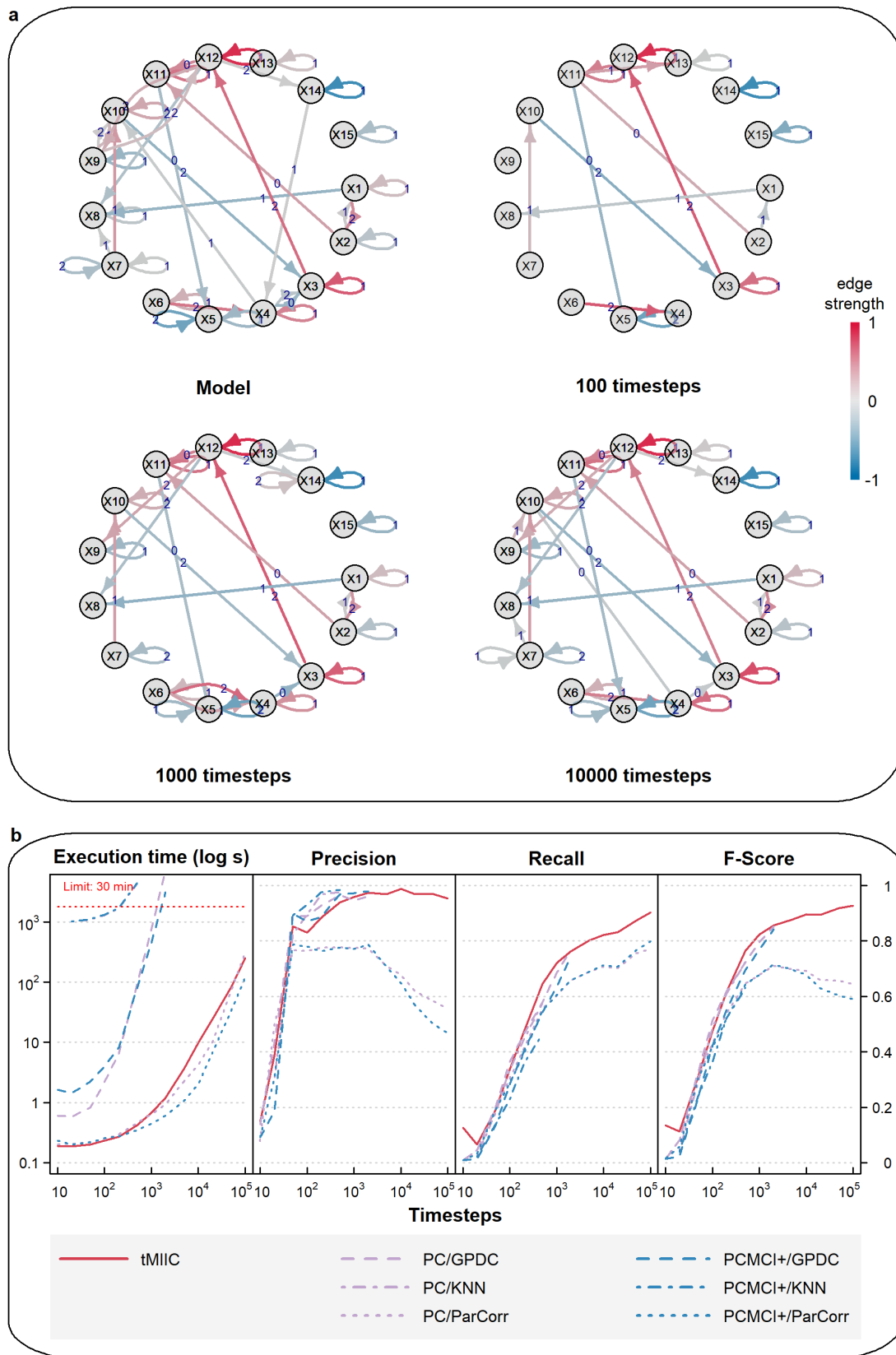
Supplementary Fig. 1. Benchmark assessment of CausalXtract's causal discovery module (tMIIC) using generated time series datasets. a , Example of a 15-node causal network to generate benchmark time series datasets based on linear combinations of contributions, Supplementary Table 1. Examples of temporal causal networks reconstructed by tMIIC based on 100, 1,000 or 10,000 simulated time steps. b , Running times and scores (Precision, Recall, Fscore) averaged over 10 datasets and compared to PC and PCMI+ methods using different kernels (GPDC, KNN, ParCorr); tMIIC is at par with PC and PCMI+ scores using GPDC and KNN kernels but runs orders of magnitude faster. Only ParCorr kernel matches tMIIC running speed but with significantly lower scores at large sample size, see Methods.
