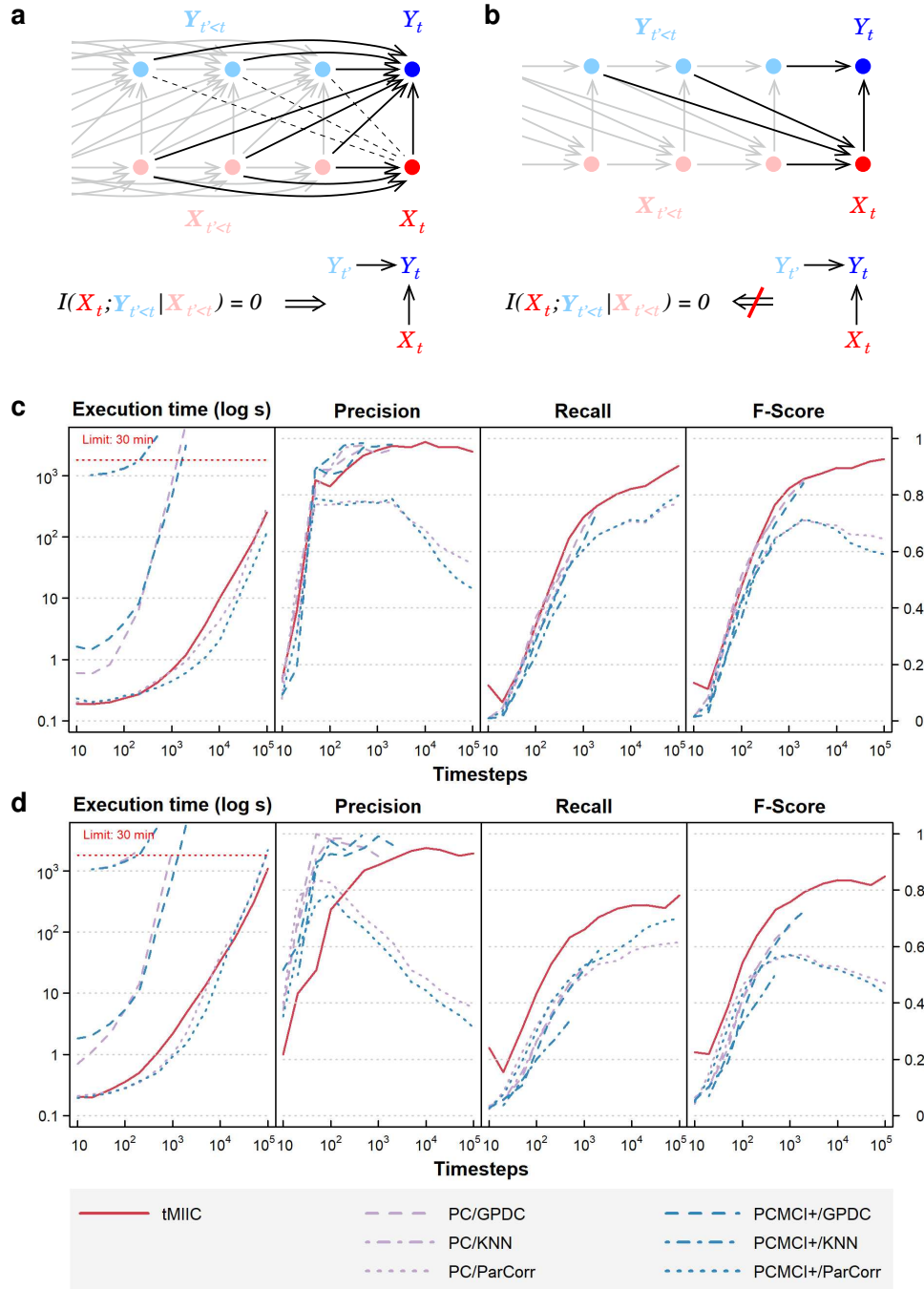
Figure 2. Relation to Granger-Schreiber temporal causality and tMIIC benchmarking against PC and PCMCi+. a , The signature of Granger-Schreiber temporal causality is a vanishing Transfer Entropy, i.e. T_{Y \rightarrow X} = I(X_t; Y_{t' < t} | X_{t' < t}) = 0 (Methods). In the time-unfolded causal network framework, it implies i ) the absence of (dashed) edge between X_t and any Y_{t'} , with t' < t , and ii ) if X_t is adjacent to Y_t , the presence of temporal (2-variable + time) v-structures, Y_{t'} \rightarrow Y_t \leftarrow X_t , for all Y_{t'} adjacent to Y_t , with t' < t (Methods, Theorem 1). b , By contrast, the presence of a temporal (2-variable + time) v-structure, Y_{t'} \rightarrow Y_t \leftarrow X_t does not imply a vanishing Transfer Entropy, as long as there remains an edge between any Y_{t' < t} and X_t . It implies that Granger-Schreiber temporal causality is in fact too restrictive and may overlook actual causal effects, which can be uncovered by graph-based causal discovery methods. Hence, tMIIC's time-unfolded network framework, combining graph-based and information-based approaches, sheds light on the common foundations of the seemingly unrelated graph-based causality and Granger-Schreiber temporal causality, while clarifying their actual differences and limitations. c , Benchmarking of tMIIC on synthetic time series datasets generated from 15-node causal networks based on linear combinations of contributions, Supplementary Table 1 and Supplementary Figs. 1-3. d , Benchmarking with more complex 15-node time series datasets based on non-linear combinations of contributions, Supplementary Table 2 and Supplementary Fig. 4. Running times and scores (Precision, Recall, Fscore) are averaged over 10 datasets and compared to PC and PCMCi+ methods using different kernels (GPDC, KNN, ParCorr).
