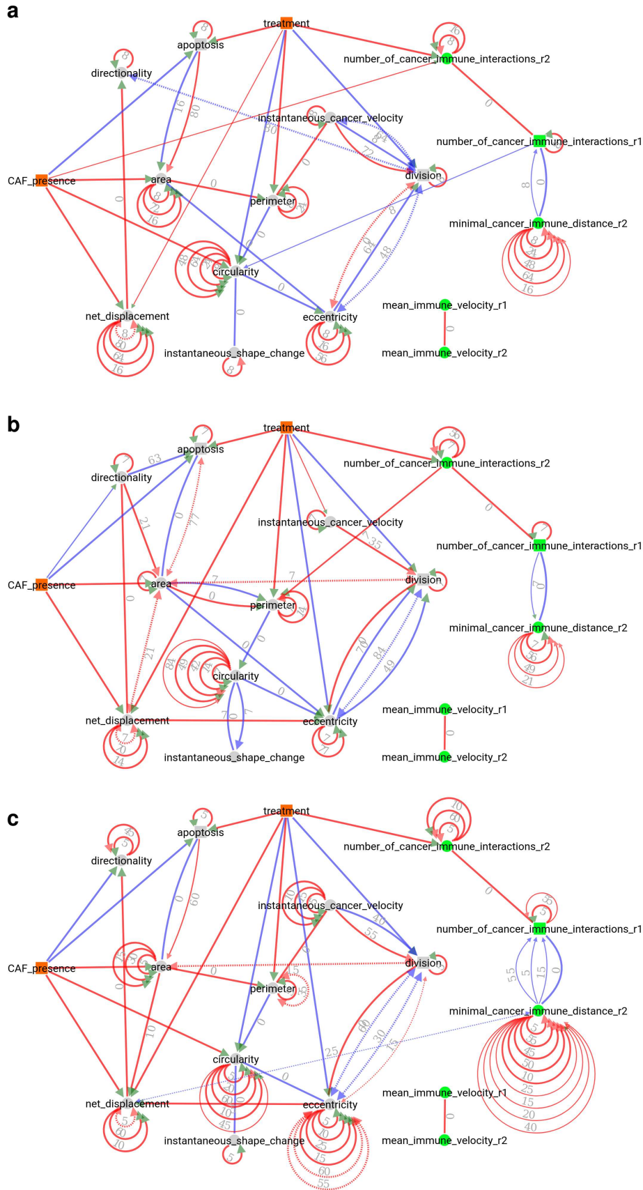
Supplementary Fig. 7. Robustness of CausalXtract’s temporal causal networks to variations in sampling rate. Summary causal networks inferred by CausalXtract using different sampling rates ( \delta\tau ). a , \delta\tau = 8 ts and \tau = 80 ts, in time step units (1 ts = 2 min). b , \delta\tau = 7 ts, and \tau = 84 ts, as chosen automatically by CausalXtract based on the average relaxation time across the 15 monitored variables, \tau_R = 40 ts, which defines a maximum lag \tau = 2\tau_R = 80 ts. Given a total number of (time-lagged and -unlagged) nodes, chosen to be around 200 nodes for computational efficiency, it leads to 13 temporal layers ( \nu + 1 = 200/15 \approx 13 ) and a lag increment \delta\tau = \tau/\nu \approx 7 ts. This summary causal network corresponds to Fig. 3a. c , \delta\tau = 5 ts and \tau = 60 ts, corresponding to \tau = \nu \cdot \delta\tau with \nu + 1 = 13 temporal layers, as in (b).
