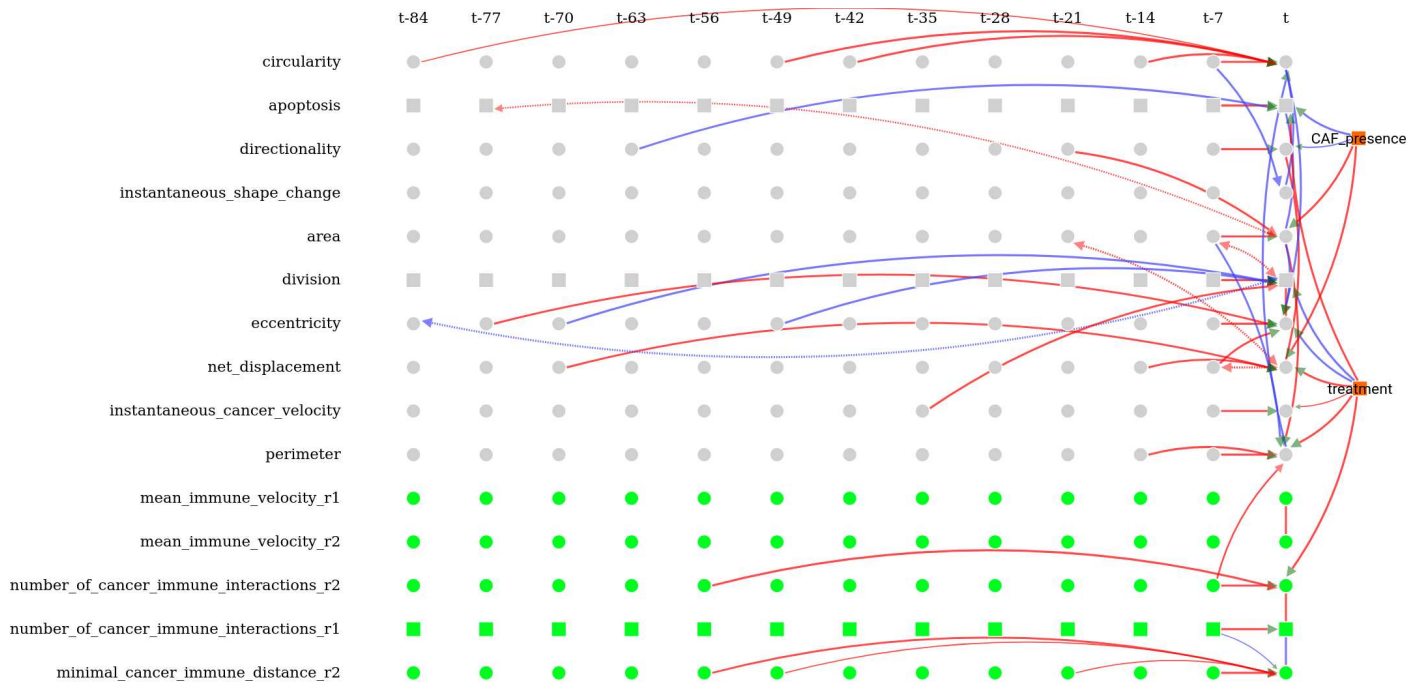
Supplementary Fig. 6. Time-unfolded causal network inferred by CausalXtract. a , Time-unfolded causal network assuming stationary dynamics of cellular ecosystems implying translational time invariance of the inferred causal network. b , Only edges involving at least one contemporaneous variables ( i.e. at time t ) need to be tested for conditional independence by tMIIC and the remaining edges are then duplicated at all previous time steps before assigning orientations when time-lagged latent variables are taken into account, Fig. 1c. Variables retaining multiple self-loops with different time-delays correspond to non-stationary variables in Supplementary Fig. 5, in agreement with benchmarks from simulated data including non-stationary variables, Supplementary Fig. 3.
