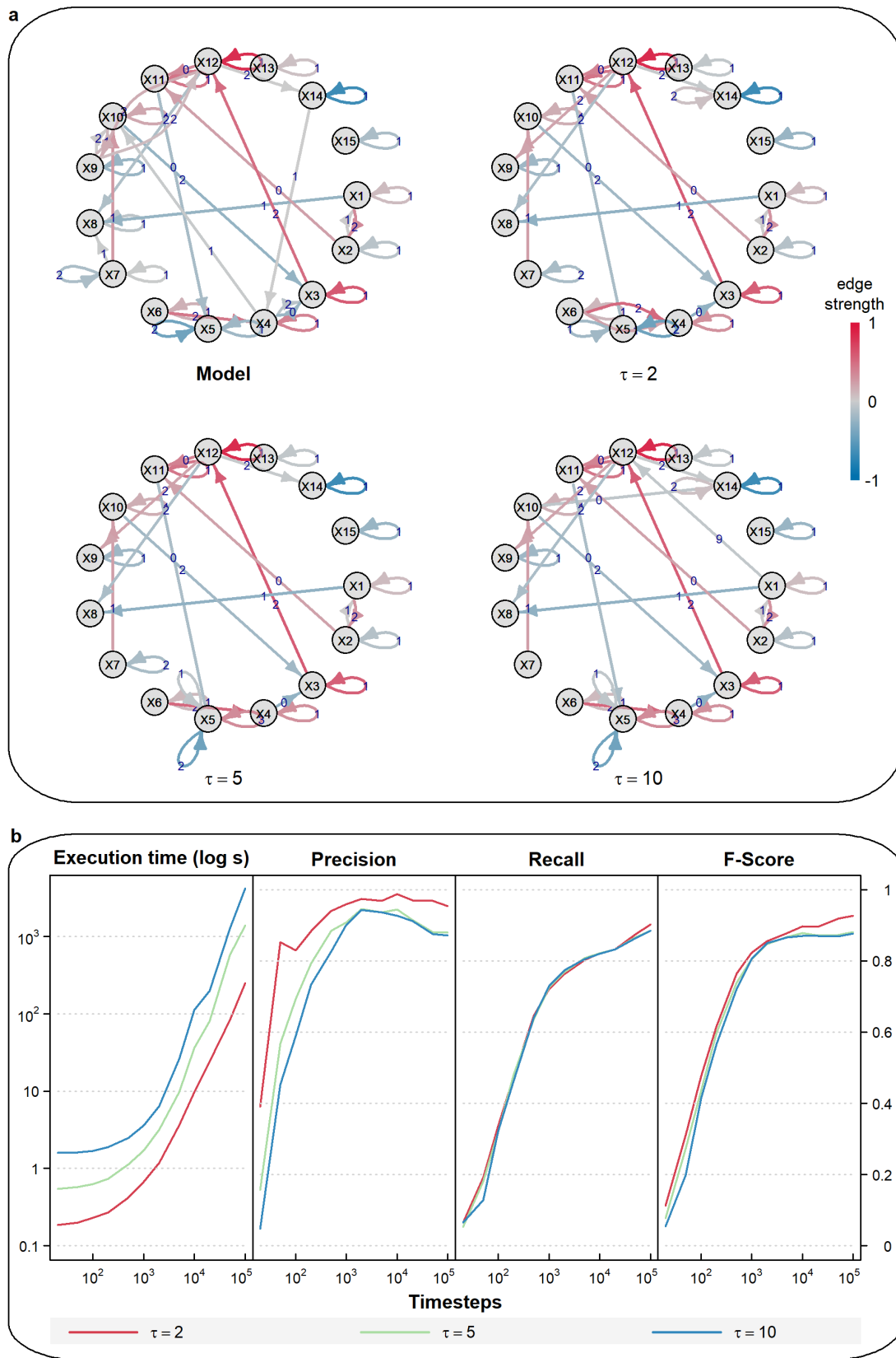
Supplementary Fig. 2. CausalXtract insensitivity to an overestimated maximum lag \tau . a, Example of a temporal causal network model with a maximum lag \tau = 2 . Corresponding temporal causal networks inferred by CausalXtract's causal discovery module (tMIIC), from 1,000 time step stationary time series (Supplementary Table 1), while assuming different maximum lags \tau = 2, 5 or 10 . b, Running times and scores (Precision, Recall, Fscore) of tMIIC temporal causal network reconstructions for \tau = 2, 5 or 10 , averaged over ten stationary time series of 10^2 to 10^5 time steps. Overestimating the maximum lag \tau has little impact on the reconstructed networks, as long as the time series are stationary, as demonstrated in Supplementary Fig. 3.
