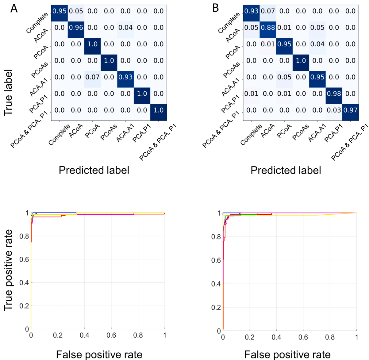
Fig. 8. Performance of the CNN (A) and MLP (B) models when trained and tested using the flow velocity waveforms in the right common carotid and vertebral arteries as input data. Confusion matrix (top) and ROC curves (bottom) for all the circle of Willis topologies. The colour code for the ROC curves corresponds to the one used in Fig. 6.
