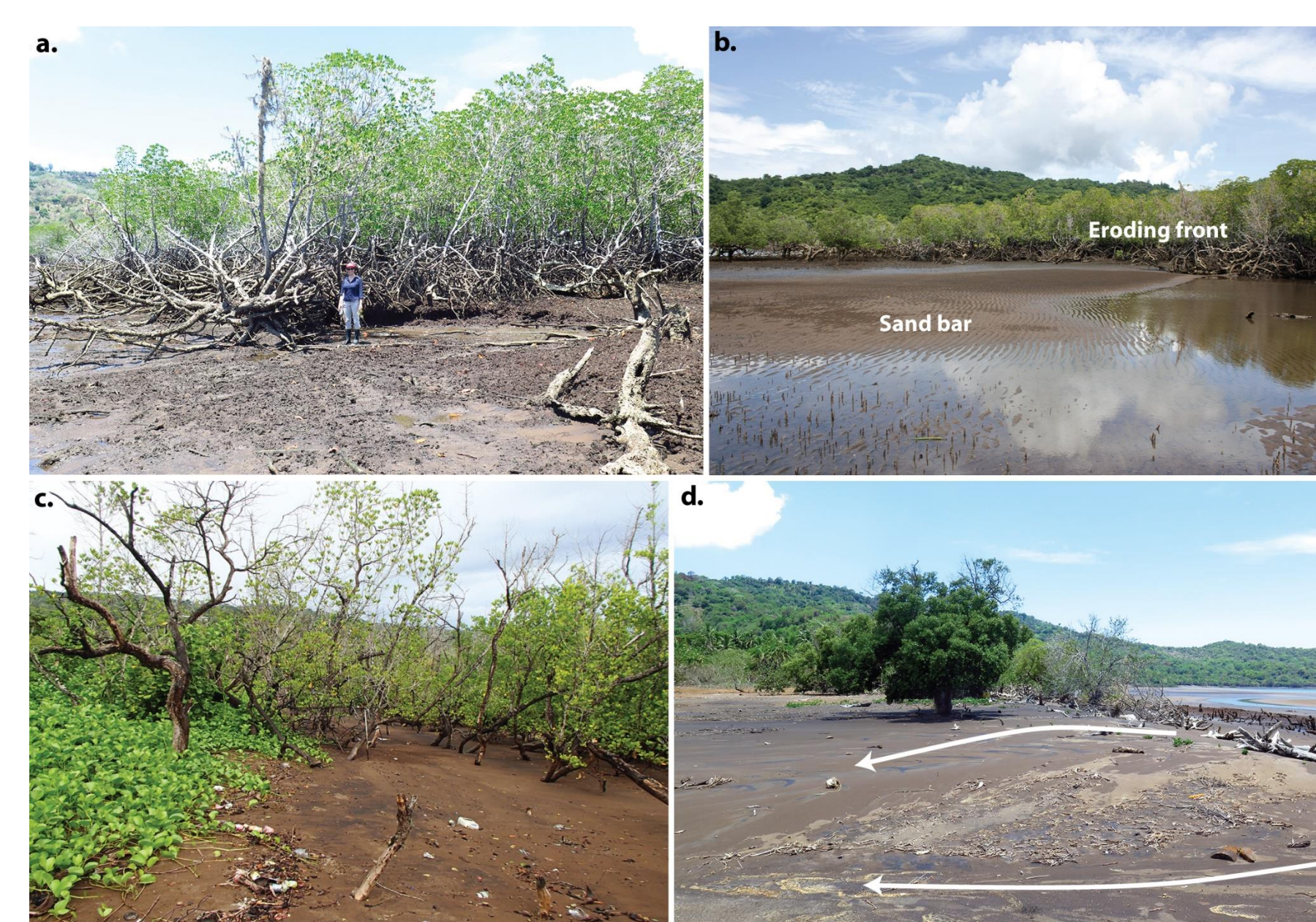
Figure 8: a. Eroding front of mature mangrove with fallen Rhizophora mucronata ; b. Sand bar near eroding front; c. Sediment burial of mangrove root systems; d. Overwash on the top of the beach ridge.
