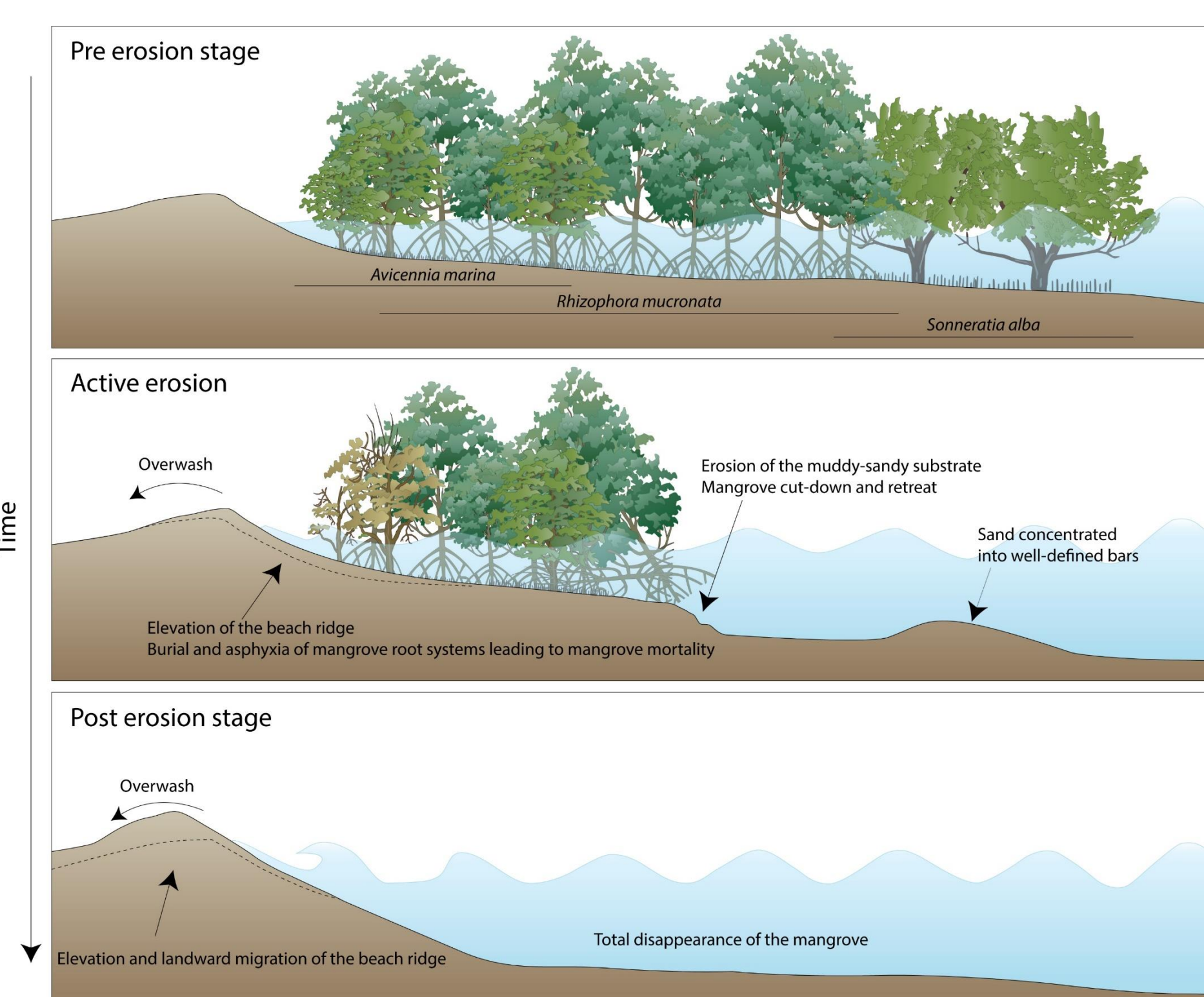
Figure 9: Model of the hydro-sedimentary reorganisation of an eroded mangrove in Mayotte
