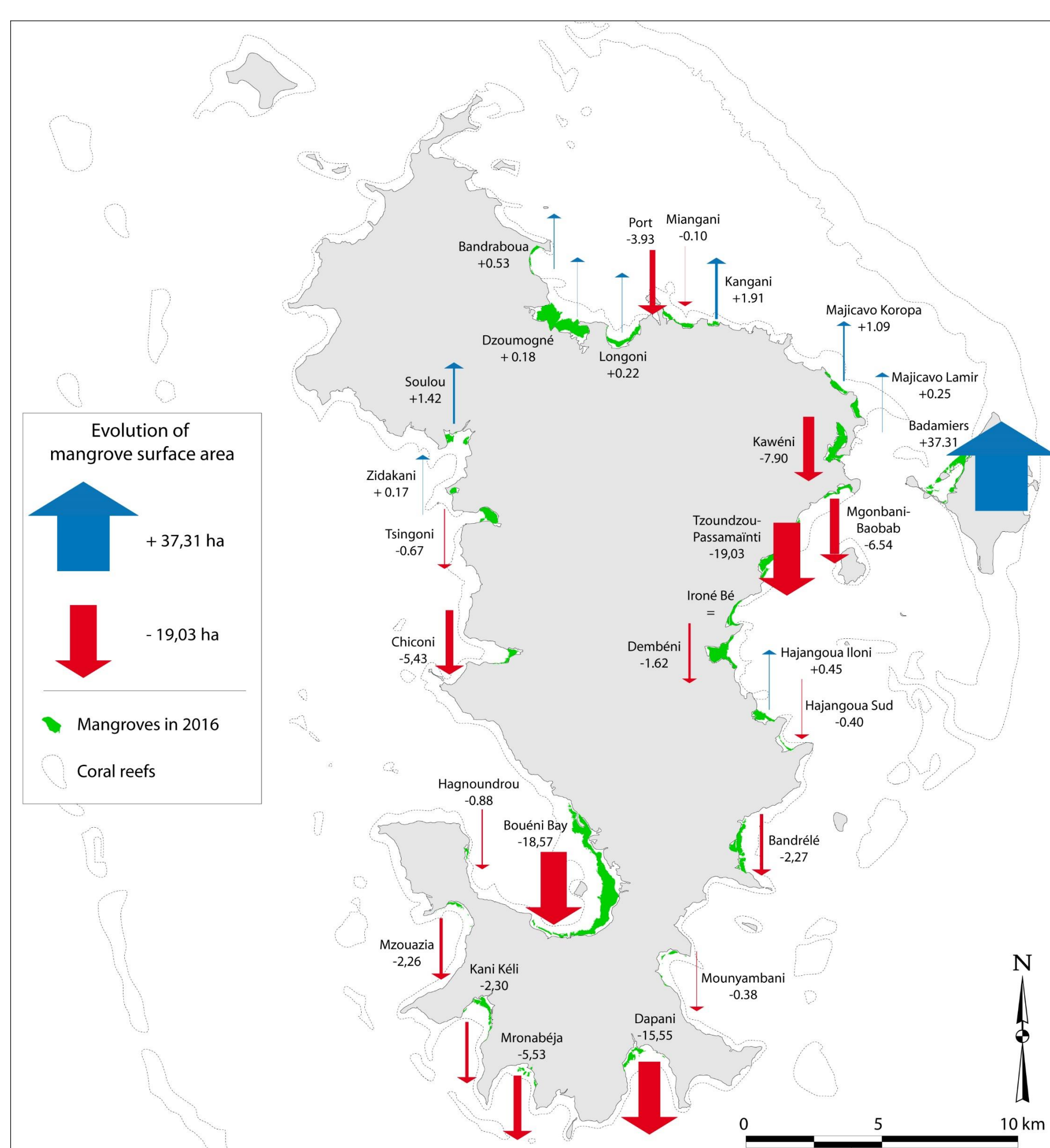
Figure 3: Overall evolution of mangroves in Mayotte between 1950 and 2016
