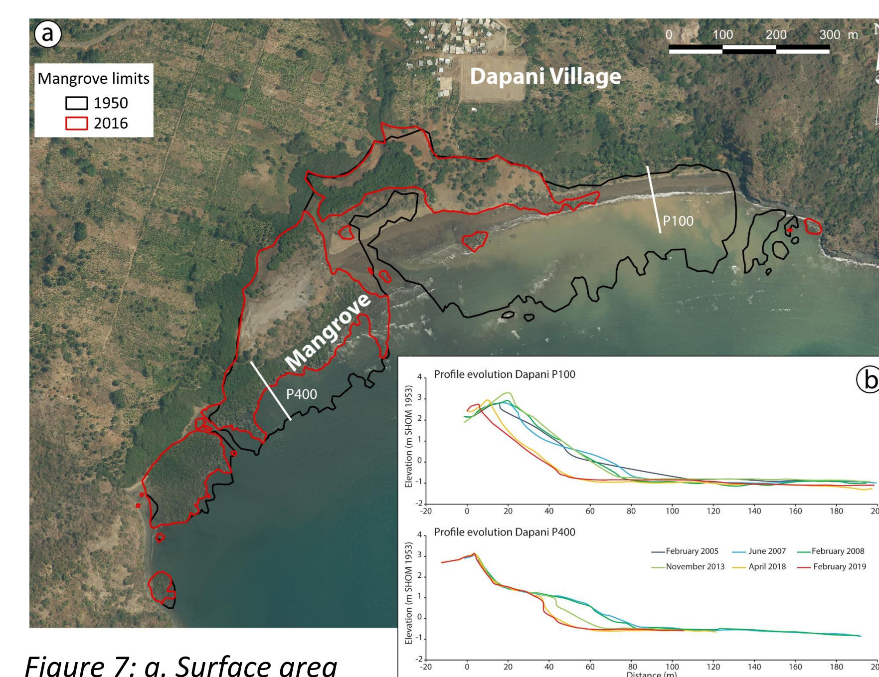
Figure 7: a. Surface area evolution of the mangrove of Dapani showing a very important regression: 1950: 27,61 ha → 2016: 12,06 ha. b. Profile changes of Dapani mangrove.
