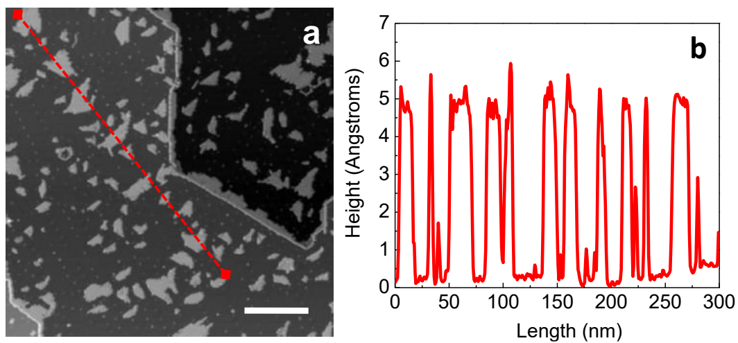
Supplementary Figure S6. Surface morphology after the 200 °C annealing step. (a) Large-scale STM topograph and (b) height profile along the dashed line in (a) showing the uniform thickness of oligomer nano-islands on the Au(111) surface. STM set-parameters are +2 V/10 pA. Scale bar is 60 nm.
