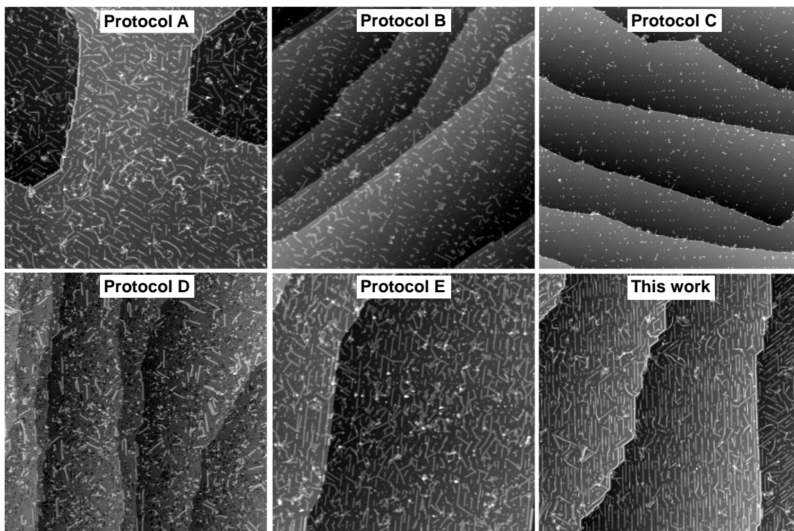
Supplementary Figure S12. Large-scale STM images showing the GNR length dispersions obtained through different on-surface protocols described in the main text, comparing with the present work (lower right STM image). Scan areas are: 300 \text{ nm} \times 300 \text{ nm} . Scan parameters are: -2 \text{ V}/10 \text{ pA} .
