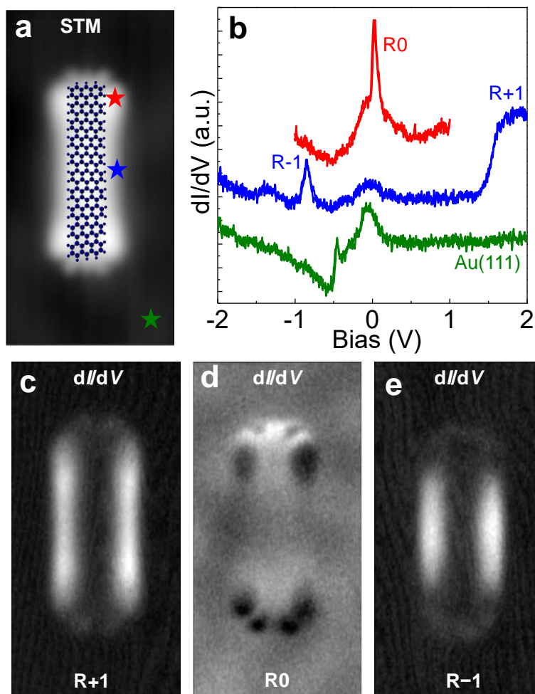
Supplementary Figure S11. dI/dV characteristics of individual GNR. (a) An STM image of a 5-monomer unit long 7-aGNR with an overlaid molecular model schematic. (b) The characteristic dI/dV tunneling spectra of 7-aGNR recorded at the spectroscopic positions marked with colored stars in (a). A characteristic Au(111) reference spectrum is also shown in green. Corresponding dI/dV maps revealing the characteristic first resonances of 7-aGNR at (c) the positive (R+1) and (e) the negative (R-1) bias voltages and, (d) the edge state resonance (R0).
