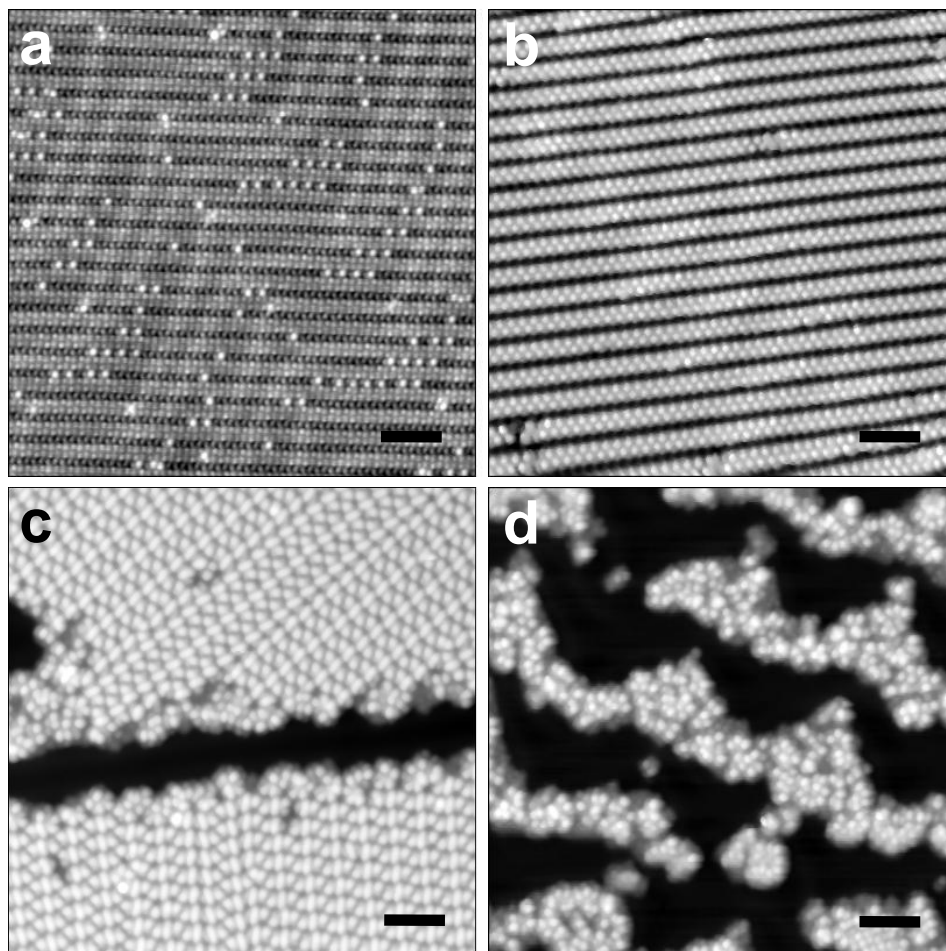
Supplementary Figure S3. Surface morphology after the 100 °C annealing step. STM topographs revealing DBBA assembly patterns in (a) ML and (b-d) bilayer (BL) regions, after annealing the 1.5 ML DBBA/Au(111) sample at 100 °C for 30 minutes. ML regions show atomic-defect-like protrusions, which originate from the physical conformational changes of individual DBBA molecules within the assembly. BL regions presented in (c) and (d) show partial reorganization of DBBA assembly differing from the initial 1D chain like structure shown in (b). STM set-parameters are +2 V/10 pA. Scale bars are 5 nm.
