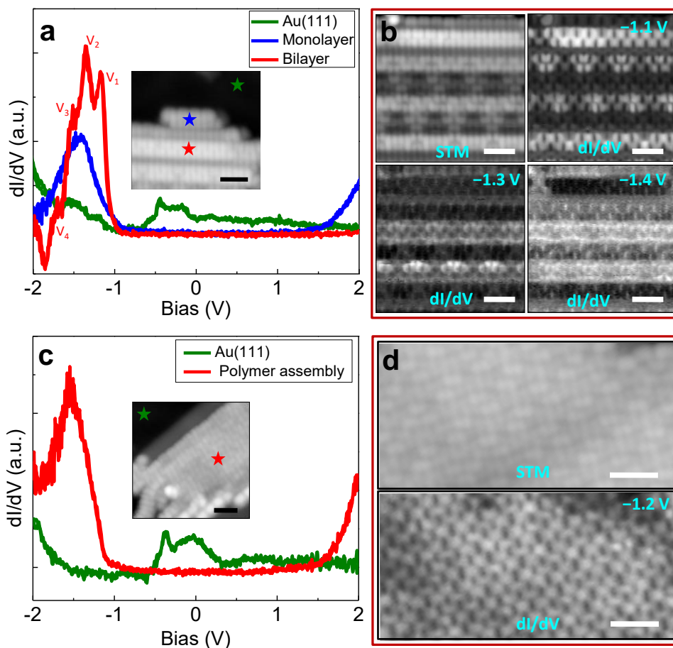
Supplementary Figure S8. Scanning tunneling spectroscopy of a polyanthyl oligomer island. (a) dI/dV spectra recorded on top of the 1 st layer (blue line) and the 2 nd layer (red line) oligomer chains of an island observed after the 200 °C annealing step. The reference dI/dV spectrum recorded on the bare Au(111) surface region is presented with a dark green line. Corresponding STS positions are marked with respective colored stars in the STM topograph presented in the inset. The vibronic satellite tunneling resonances ( V_1 , V_2 , V_3 , and V_4 ) from the 2 nd layer oligomer chain are labeled in the dI/dV plot. (b) dI/dV maps recorded at three different voltages (-1.1 V, -1.3 V and -1.4 V) suggest the vibronic origin of the satellite peaks. (c) dI/dV spectrum (red) and (d) map recorded from a polyanthyl oligomer island after the 250 °C annealing step. The reference dI/dV spectrum in green is identical to the green plot in (a). No vibronic satellite peaks from oligomer chains are observed but the spectrum is identical to the blue plot in (a), implying that the oligomer island has converted to a single layered configuration. STM set-parameters are -2 V/10 pA for the STM images given in the insets of (a) and (c), -1.1 V/100 pA for (b) and -1.2 V/100 pA for (d). Scale bars are 2 nm.
