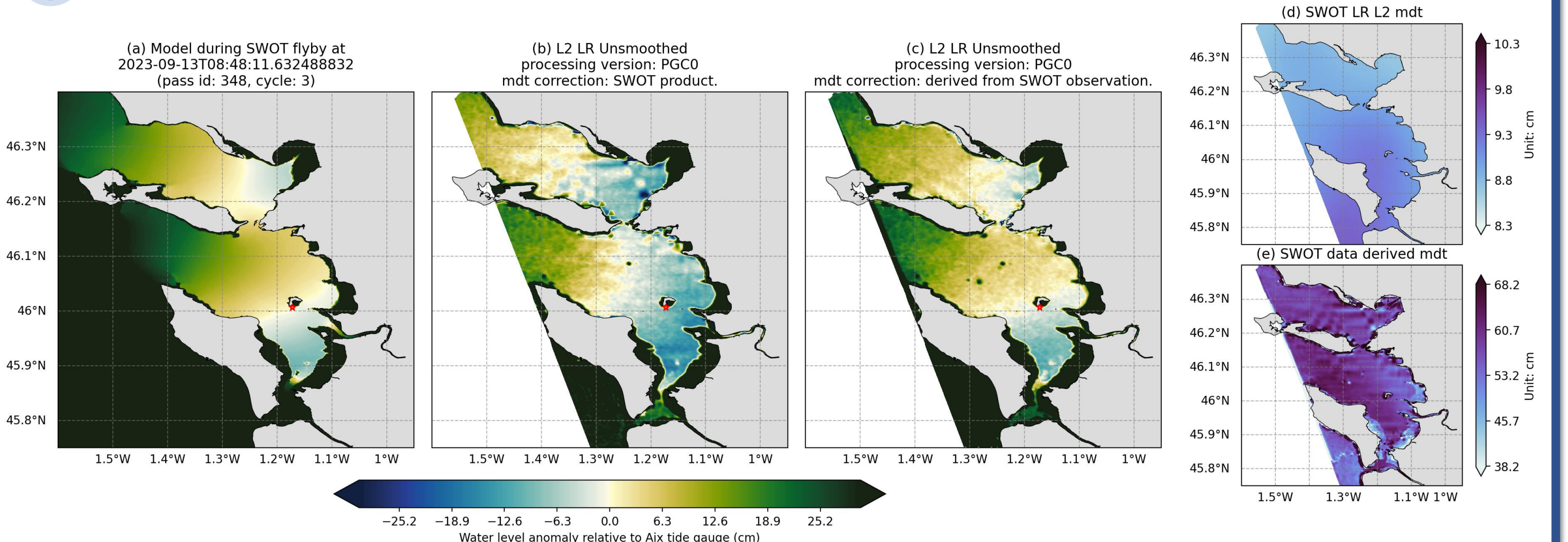
Fig 6: Coastal SSHA gradient from model (a) and SWOT (b, c) relative to Aix island tide gauge location (red star). SSHA in (b) and (c) are computed using Eqn 1. Mean dynamic topography (mdt) correction used in (b) is from SWOT L2 product (d) and correction used in (c) is computed with 15 cycles of SWOT data (e) using Eqn 2, which includes mdt and stationary SWOT artifacts.
