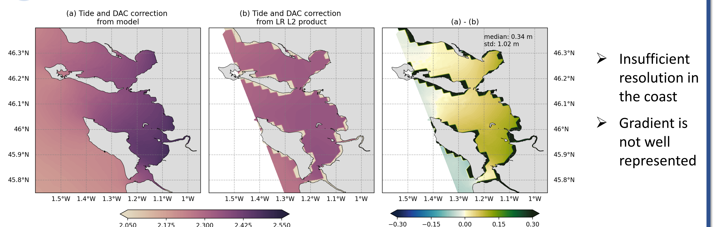
Fig 5: Tide and dynamic atmospheric correction (dac) from regional model (a) and from SWOT LR level 2 product (b) and their comparison.
