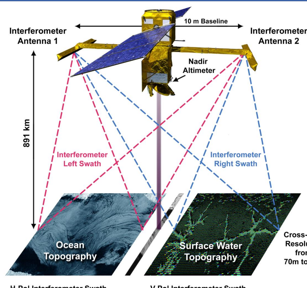
Fig 2. Diagram of SWOT Data Collection https://swot.jpl.nasa.gov/resources/104/diagram-of-swot-data-collection/
