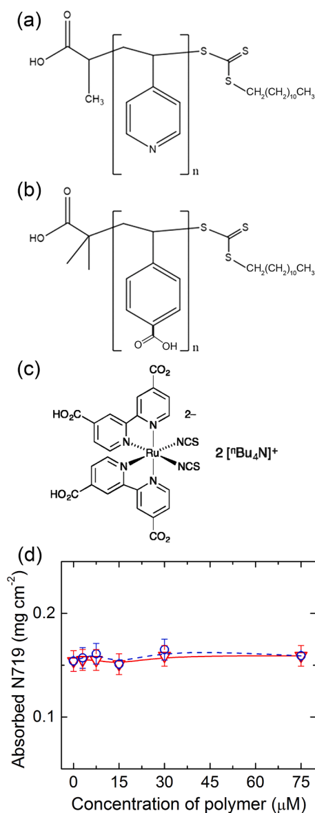
Fig. 2. Molecular structures of the P4VP (a), PVBA (b), and N719 dye (c). Amount of the adsorbed dye in the mesoporous titania vs. polymer concentration for sequential adsorption of P4VP (red triangles) and PVBA (blue circles) (d).
