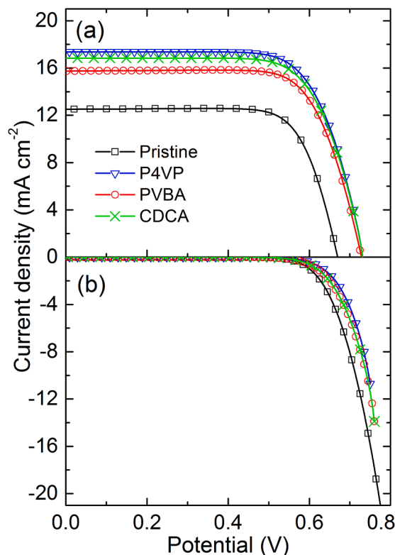
Fig. 5. I - V curves under 1- Sun equivalent (a) and in the dark (b) of the DSSCs with pristine TiO 2 /dye photoanode (squares); after co-adsorption of P4VP (triangles), PVBA (circles) or CDCA (crosses).
