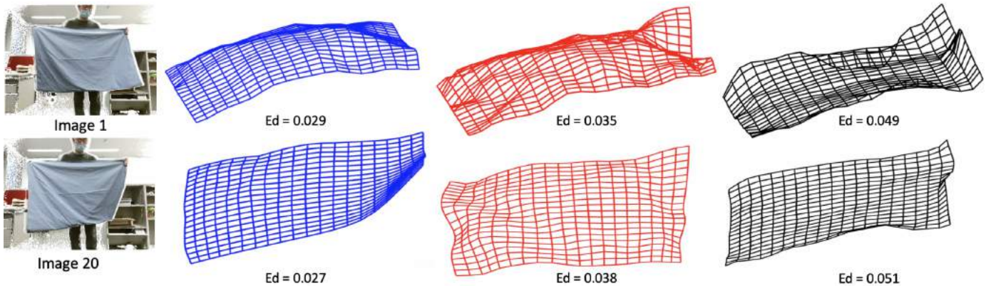
Fig. 7: Blue Sheet dataset . Reconstructed surfaces for two images. The predictions of Ours are shown in blue, of Pa21-R in red, and of An17 in black. Note that our reconstructions are less noisy and match the surface 3D shape much better.
