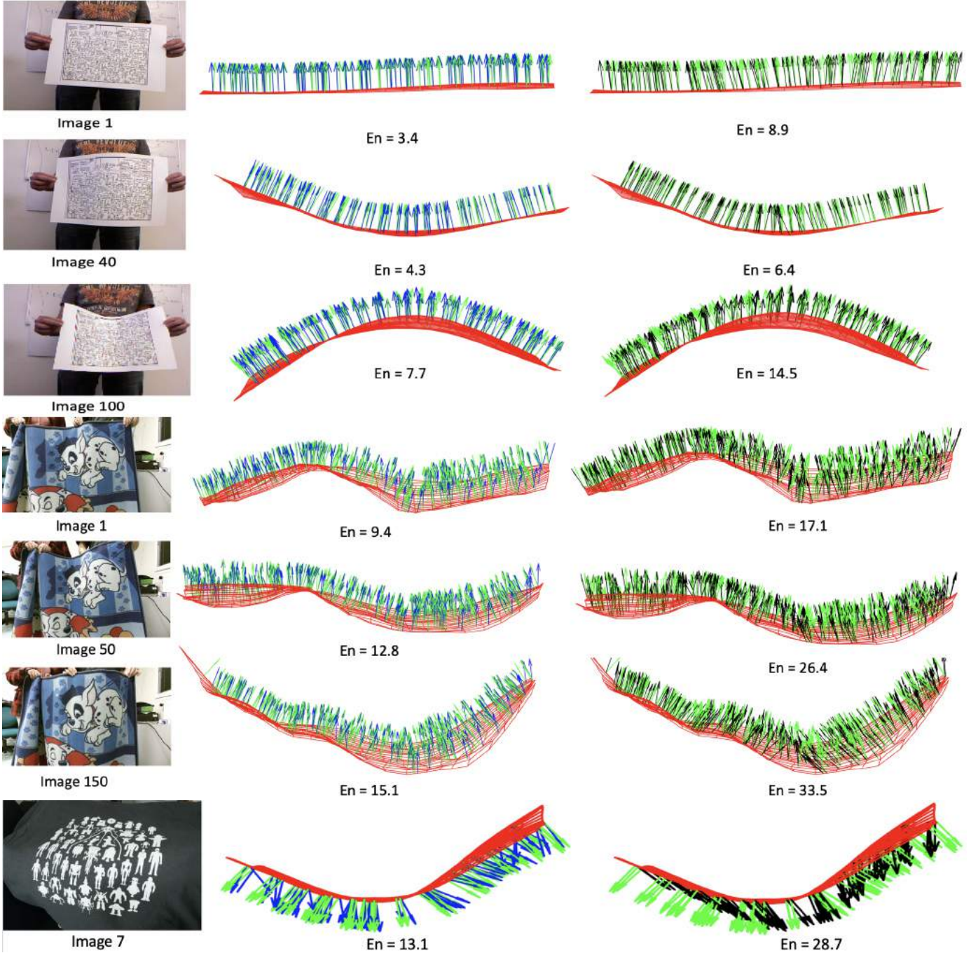
Fig. 5: Datasets used in our previous work. Reconstructed normals on three images. The ground-truth normals are shown in green, the ones predicted by Ours in blue, and those by Pa21-R in black. Note that our normals are far less noisy.
