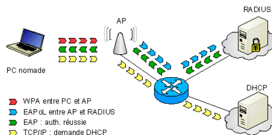
Figure 3 - Architecture WPA
