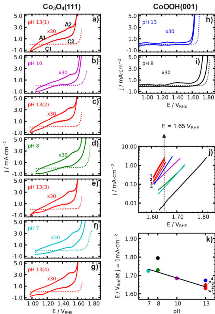
Figure 3. Cyclic voltammograms (dotted lines) of the (a-g) Co 3 O 4 and (h, i) CoOOH catalyst in electrolytes of different pH (sweep rate 5 mV/s, for Co 3 O 4 and 10mV/s for CoOOH, iR-corrected). To show the CV in the pre-OER regime the current density was multiplied by a factor 30 (solid lines). (j) Tafel plots in the OER region, extracted from the iR-corrected potential scan in positive direction of the CVs. For pHs 7 and 8, the pseudo-capacitive current was subtracted. For the 4 measurements at pH 13 the number of the measurement in the sequence is given. (k) pH dependence of the OER overpotential at a constant current density of 1 mA/cm 2 .
