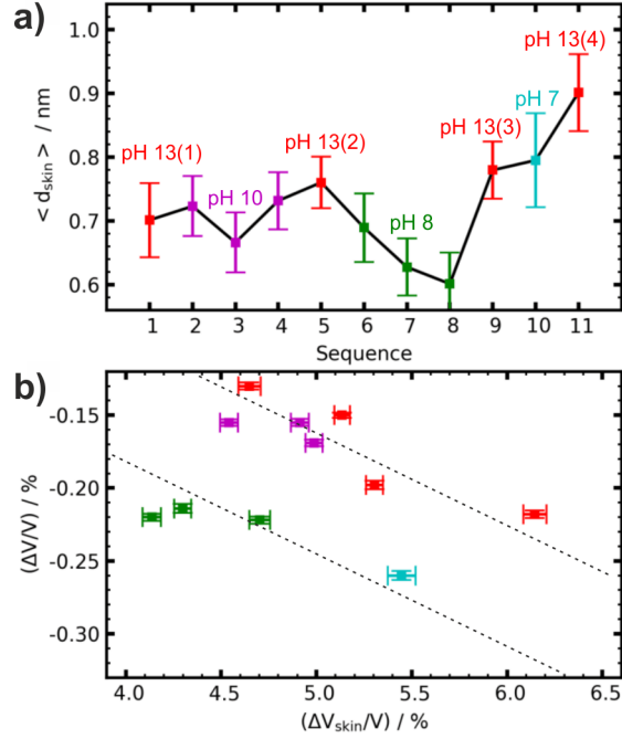
Figure 8. Effect of pH and time on the structural changes between 1.05 to 1.6 V_{RHE} . (a) Evolution of average skin layer thickness \langle d_{skin} \rangle over the course of the experiment. (b) Relative change of the unit cell volume in the spinel lattice of the \text{Co}_3\text{O}_4 grains as function of the fraction of the oxide that is converted into the skin layer. Dashed lines indicate the linear relationship found in Ref. [17] at pH 13.
