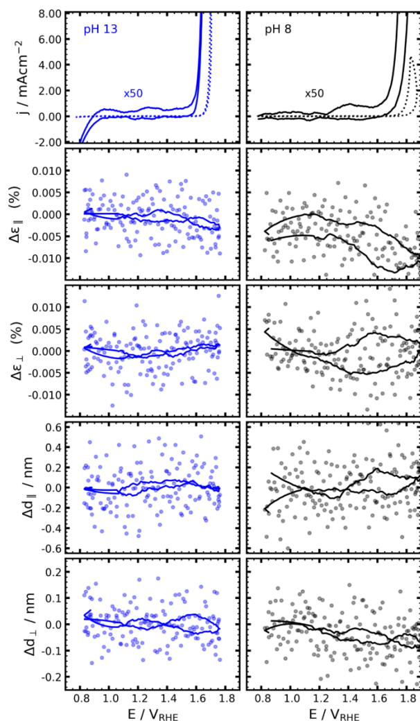
Figure 4. Operando SXR D results, showing the structural changes in a CoOOH(001) film on Au(111) during three potential cycles at pH 13 and pH 8 (scan rate 10 mV/s). Each column displays (from top to bottom) the electrochemical current density j and the variations of the horizontal strain \Delta\varepsilon_{\parallel} , the vertical strain \Delta\varepsilon_{\perp} , the horizontal crystallite grain size \Delta d_{\parallel} , and the vertical crystallite grain size \Delta d_{\perp} . The data were obtained from the variation of the CoOOH(017) Bragg reflection during the CVs shown in the upper panel
