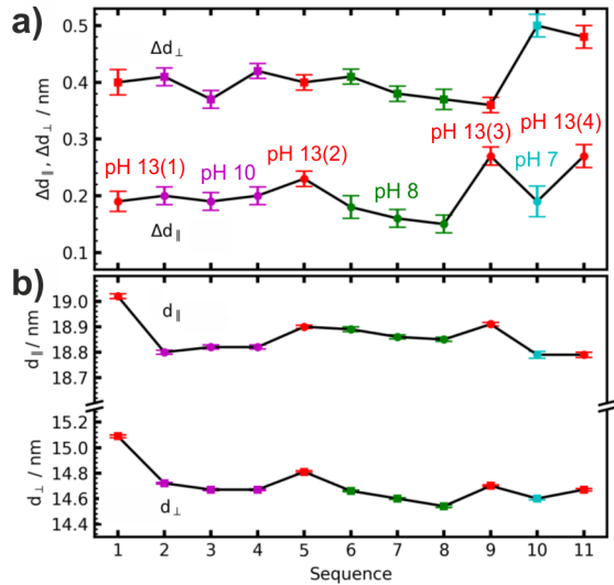
Figure 6. (a) Potential-dependent changes in horizontal and vertical grain size \Delta d_{\parallel} and \Delta d_{\perp} between 1.05 and 1.6 V and of (b) the absolute horizontal and vertical grain sizes d_{\parallel} and d_{\perp} at 1.05 V over the course of the experiment. At each point in the sequence 2-3 consecutive potential cycles of the type shown in Figure 5 were recorded. Results for the positive and negative scan were averaged to reduce the effect of the hysteresis.
