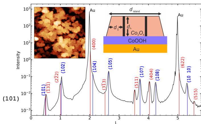
Figure 2. Structure and morphology of the \text{Co}_3\text{O}_4 model electrocatalysts. X-ray scattering intensity profile along the (01L) crystal truncation rod of \text{Au}(111) . Two sharp Bragg peaks ( L=2, 5 ) of the \text{Au} substrate are coexistent with weaker Bragg peaks, which are assigned to the epitaxial \text{Co}_3\text{O}_4 (red) and underlying \text{CoOOH} (blue) deposits. The Miller indices given for each Bragg peak refer to the conventional unit cells of \text{Co}_3\text{O}_4 (fcc) and \text{CoOOH} (hcp). In addition, a characteristic AFM image ( 1 \times 1 \mu\text{m}^2 ) of the as-prepared film surface and a model illustrating the structural parameters are included as insets.
