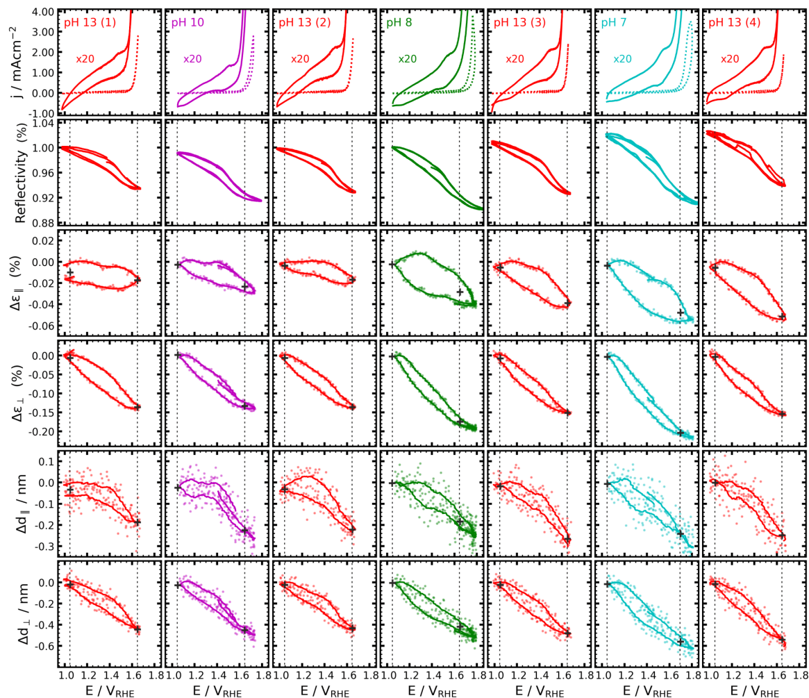
Figure 5. Operando SXR D results, showing the structural changes in a \text{Co}_3\text{O}_4(111) film on \text{Au}(111) in electrolytes of different pH during cyclic voltammograms (scan rate 5 mV/s). The data were recorded on the same \text{Co}_3\text{O}_4 sample and are selected from the full dataset (Figure S1). They are displayed in the figure (from left to right) following the measurement sequence. Each column shows (from top to bottom) the electrochemical current density j , with the double-layer region being scaled by a factor of 20 for better visibility (solid lines), the optical reflectivity, normalized to the initial value of the as prepared sample, and the variations of the horizontal strain \Delta\varepsilon_{||} , the vertical strain \Delta\varepsilon_{\perp} , the horizontal crystallite grain size \Delta d_{||} , and the vertical crystallite grain size \Delta d_{\perp} . The structural data were obtained from the variation of the \text{Co}_3\text{O}_4(1\bar{1}3) Bragg reflection during the CVs shown in the upper panel and are given versus the iR-corrected potential. Potentials and values used for the data given in table 1 are marked by dashed lines and crosses, respectively.
