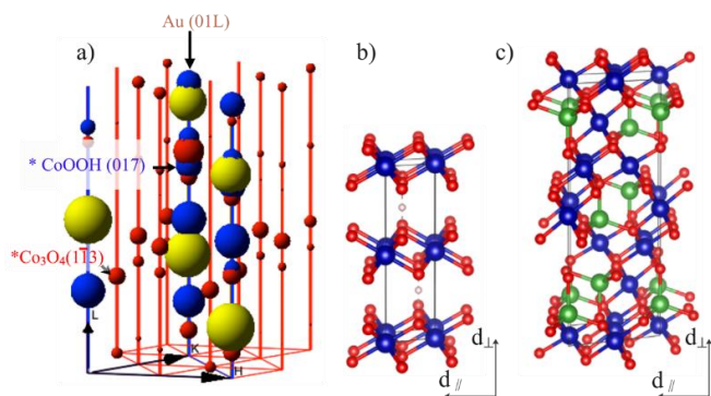
Figure 1. a) Reciprocal space geometry of Bragg peaks (spheres) and crystal truncation rods for Au(111) (yellow), the epitaxial \text{Co}_3\text{O}_4(111) film (red), and the epitaxial \text{CoOOH}(001) film (blue). The relative scattering intensities of the Bragg peaks are illustrated by the diameters of the spheres. In the employed hexagonal coordinate system the L axis is parallel to the Au[111] lattice vector, while the H and K axes are within the Au(111) plane. Within the surface plane, the \text{Co}_3\text{O}_4[2\bar{2}4] and the \text{CoOOH}[100] lattice vector are aligned with the H axis. Two Bragg peaks used for the operando studies, \text{Co}_3\text{O}_4(1\bar{1}3) and \text{CoOOH}(017) , are highlighted. (b,c) Crystal structures of (b) \text{CoOOH} and (c) \text{Co}_3\text{O}_4 , with \text{Co}^{3+} atoms shown in blue, \text{Co}^{2+} atom in green, O atoms in red, and H atoms in white. In the chosen unit cells, the c axes are oriented along the surface normal for \text{CoOOH}(001) and \text{Co}_3\text{O}_4(111) epitaxial films (adapted from Ref. 16. Copyright American Chemical Society 2019).
