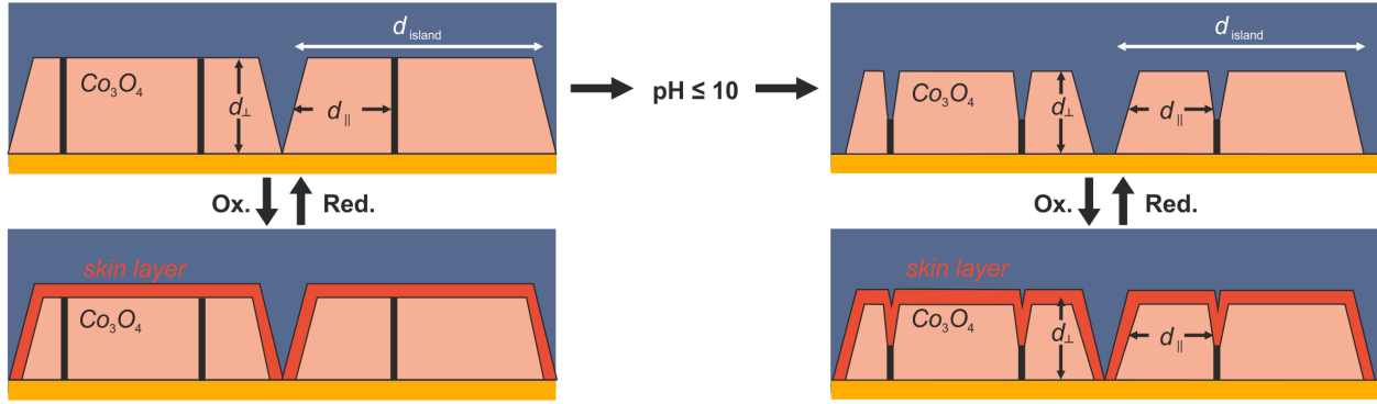
Figure 9. Schematic illustration of the evolution of the \text{Co}_3\text{O}_4 film morphology upon potential cycles at pH 13 (a) and pH \leq 10 (b). At pH 13 the morphology stays stable. At lower pH irreversible Co dissolution promotes surface roughening and concomitant increases in skin layer volume.
