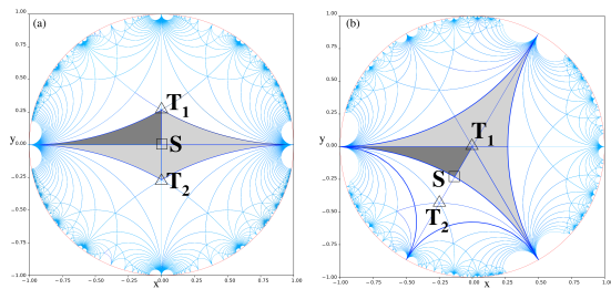
FIG. 3. Stereographic projection on a Poincare disk of the configurational space of metric tensors \mathbf{C} with \det \mathbf{C} = 1 given by the formulas x = t(C_{11} - C_{22})/2 , y = tC_{12} , where t = 2(2 + C_{11} + C_{22})^{-1} , see [80] for details. In (a,b) the reference states are the square phase S and the triangular phase T_1 , respectively. Dark gray indicates the minimal periodicity domain, light gray – the minimal elastic domain; blue lines represent the tessellation induced by the GL(2, \mathbb{Z}) global symmetry.
