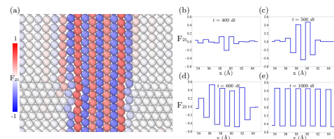
FIG. 7. (a) Layer-by-layer propagation of the deformation gradient (here only F_{21} component) during S-T transformation; (b-e) transient spatial configurations of the deformation gradient showing the formation of an ideally periodic pattern.
