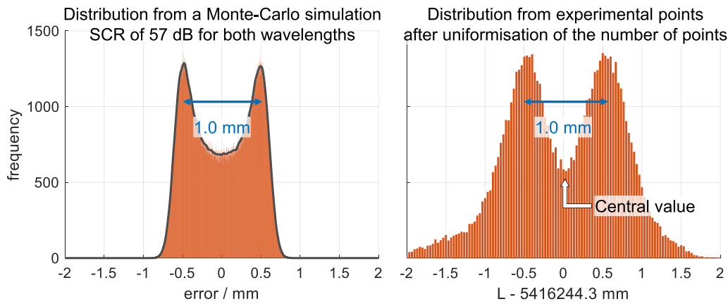
Figure 23. Comparison of the simulated and experimental distributions of the air-index compensated distances measured over 5.4 km as for a received RF power as low as -15 dBm and considering only the telemetric contributions.
