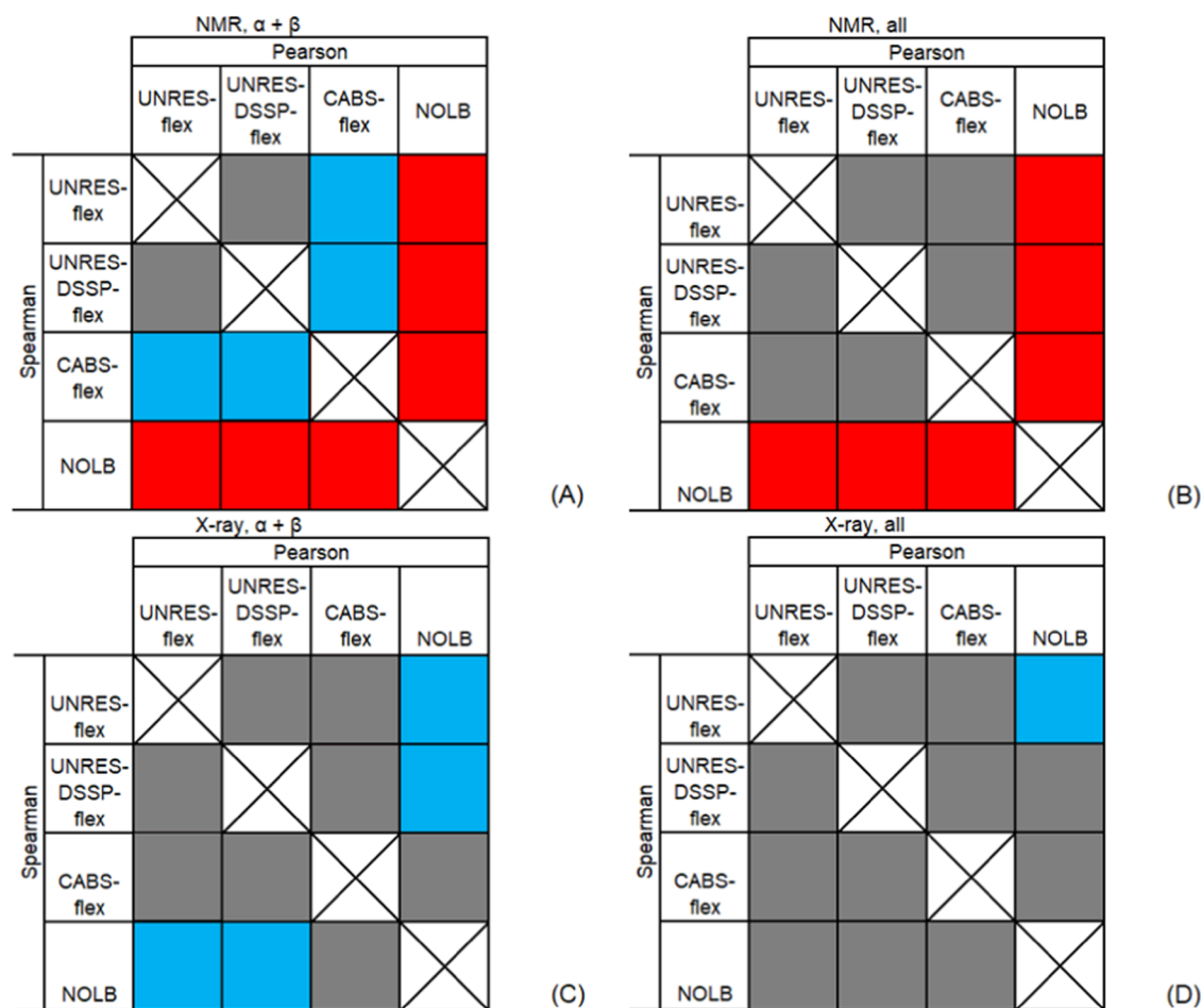
Figure 4. Visualization of the sign of and statistical significance of the r_p (above-diagonal) and r_s (below-diagonal) correlation coefficients corresponding to the four methods of fluctuation prediction evaluated in this work for NMR (A, B) and X-ray (C, D) structures and \alpha + \beta (A, C) and all (B, D) proteins. For r_p , the method corresponding to the respective column heading is compared with that of an above-diagonal row entry, while for r_s , the method corresponding to the respective row heading is compared with that of a below-diagonal column entry. Red: the difference is negative at <0.05 significance level, blue: the difference is positive at <0.05 significance level, and gray: the difference is statistically insignificant.
