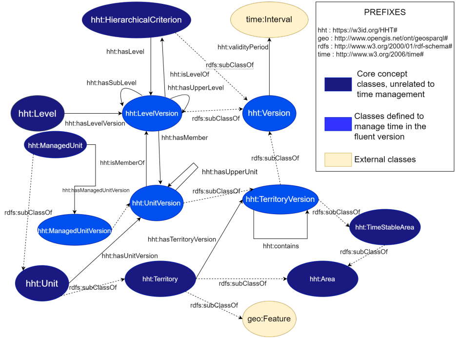
Fig. 1: HHT core classes and properties
