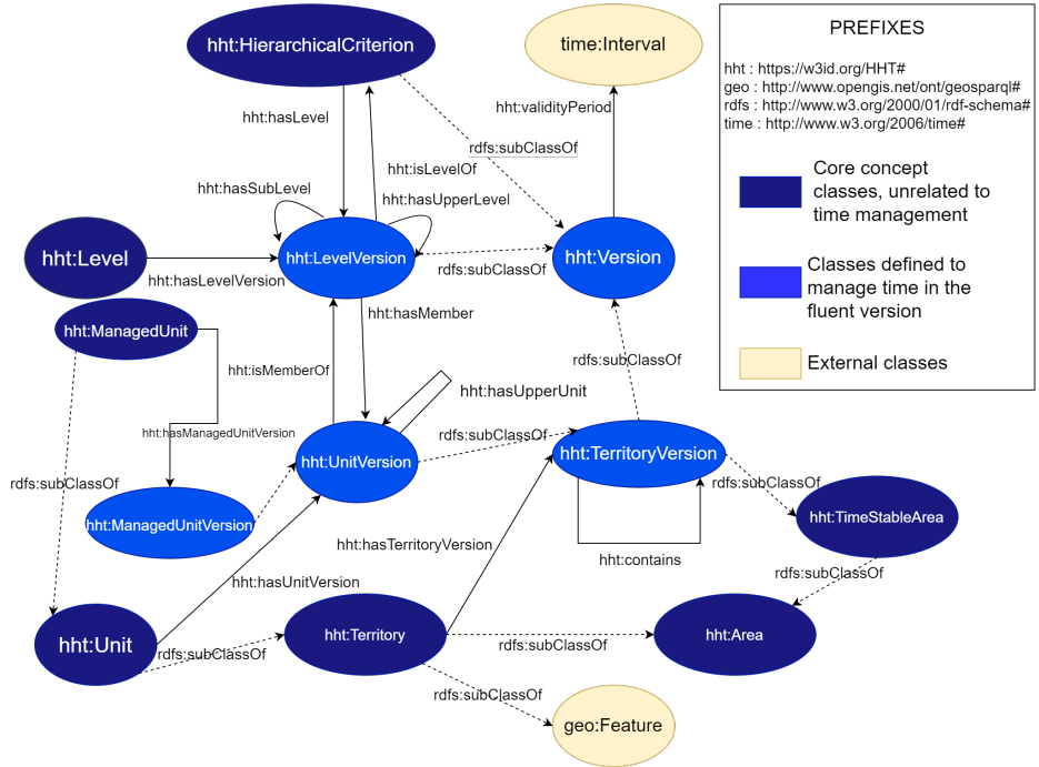
Fig. 1: HHT core classes and properties
