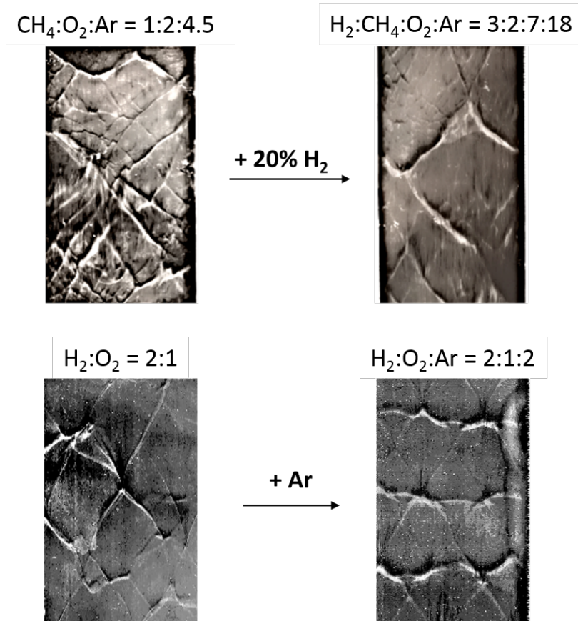
Figure 5: Effect of the mixture composition on the cellular structure and regularity. The top pair is for mixtures with \text{CH}_4 as part of the fuel mixtures, at the initial pressure of 180 mbar. The bottom set is for mixtures with \text{H}_2 as the fuel, at the initial pressure of 180 mbar/150 mbar.
