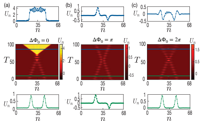
FIG. 4. Identical breathers with amplitude (A_{\text{br}}, \omega_{\text{br}}, qa) = (0.95, 1.339, 0.32) and relative phase difference (a) \Delta\Phi_0 = 0 , (b) \Delta\Phi_0 = \pi and (c) \Delta\Phi_0 = 2\pi , respectively, counter-propagating in a lattice of N = 69 elements. In (b) a nearly elastic collision is observed in contrary to (a) and (c) in which radiation and high-amplitude excitations are generated. The vertical lines correspond to the spatial profile of system as depicted in the panels.
