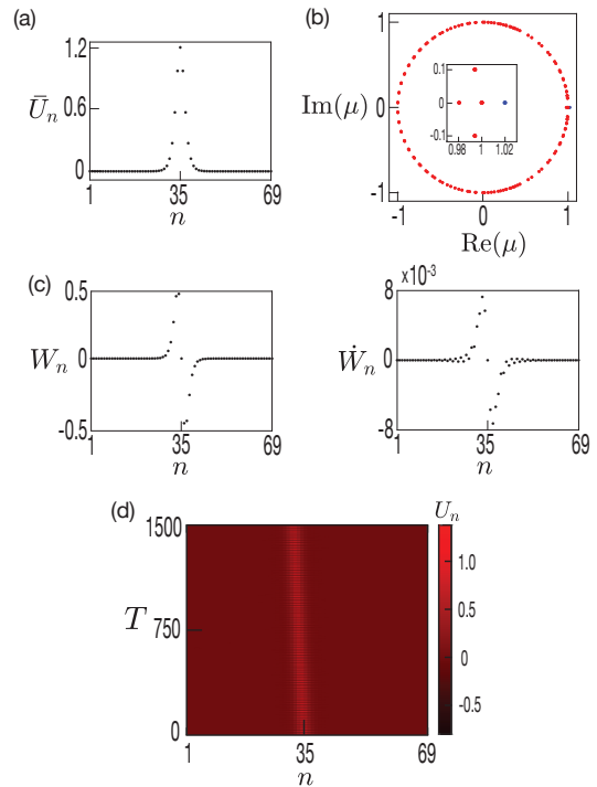
FIG. 10. (a) A discrete breather with frequency \omega_{\text{br}} = 1.26 and (b) the corresponding Floquet multipliers on the complex plane. The inset indicates the presence of a Floquet multiplier outside the unit circle leading to a real instability. (c) The displacement and velocity profile of the eigenvector which corresponds to the unstable Floquet multiplier of the solution with frequency \omega_{\text{br}} = 1.26 . By perturbing the discrete breather using the eigenvector a moving one is obtained as can be reported in (d).
