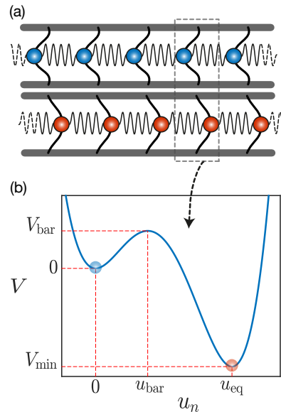
FIG. 1. (a) Schematic representation of the considered chain of linearly coupled bistable elements. The filled circles represent the masses and the curved black lines the buckled beams that are bistable. (b) The potential produced by the buckled beams and described by Eq. (2) for V_2 > 0 . The blue and the red filled circles correspond to masses placed in the local and the global equilibrium point of the potential, respectively.
