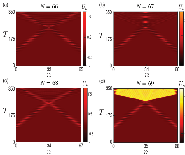
FIG. 5. Two in-phase breathers with (A_{\text{br}}, \omega_{\text{br}}, qa) = (0.95, 1.339, 0.32) counter-propagate and collide within lattices with different lengths. The breathers' parameters are chosen such as v_{\text{br}} \approx \omega_{\text{br}}/2\pi . In (a) and (c) the formation of new counter-propagating localized wave-packets is observed. In (b) and (d) energy trapping and formation of transition fronts, respectively, are observed indicating that depending on the phase, the outcome can significantly change.
