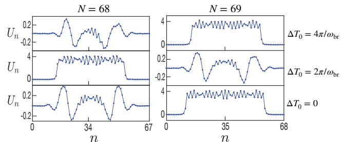
FIG. 6. Snapshots of displacements U_n in a lattice consisting of N = 68 elements (left panel) and N = 69 (right panel), respectively, after the collision of identical breathers with amplitude (A_{\text{br}}, \omega_{\text{br}}, qa) = (1.00, 1.32, 0.32) . The breathers have been generated with time difference \Delta T_0 and counter-propagate. From down to top the time difference equals to \Delta T_0 = \{0, T_{\text{br}}, 2T_{\text{br}}\} , respectively. We show that a transition wave is always triggered if we appropriately tune the time difference \Delta T_0 . As observed, the tuning depends on the lattice length.
