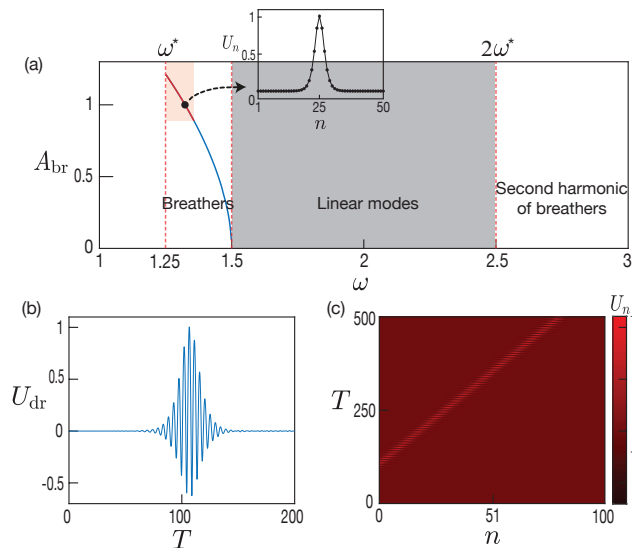
FIG. 2. (a) Frequency regimes where breathers, linear modes and breather’s second harmonic are predicted. The breather’s amplitude A_{\text{br}} as function of frequency is also depicted. In the inset, the spatial profile of a breather with frequency \omega_{\text{br}} = 1.32 (black marker) is shown. (b) Time evolution of the displacement imposed to a driven unit to excite the breather. (c) Propagation along a lattice of N = 101 elements of the moving breather produced by the driving profile depicted in (b). The breather’s characteristics are (A_{\text{br}}, \omega_{\text{br}}, qa) = (1.00, 1.32, 0.3) .
