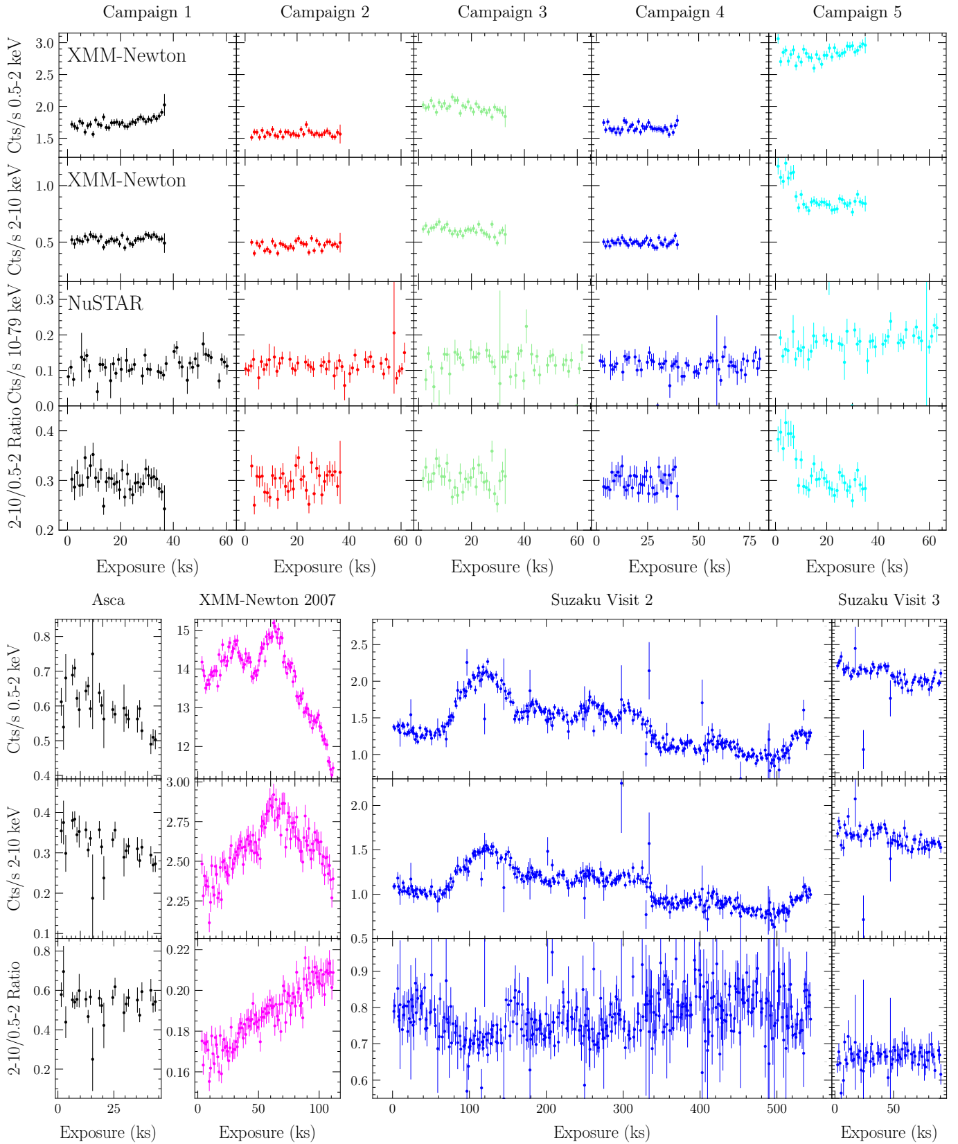
Fig. 2. ESO511-G030 light curves. Top panels: Background-subtracted light curves from the 2019 multi-wavelength campaign. The first and second row refer to the XMM-Newton 0.5–2 and 2–10 keV bands, respectively, while the last row shows the ratios between the two bands. The NuSTAR light curves extracted in the 10–79 keV band are also shown. Bottom panels: Background-subtracted time series for ASCA (black), the 2007 XMM-Newton orbit (red) and the Suzaku visits two and three (in blue).
