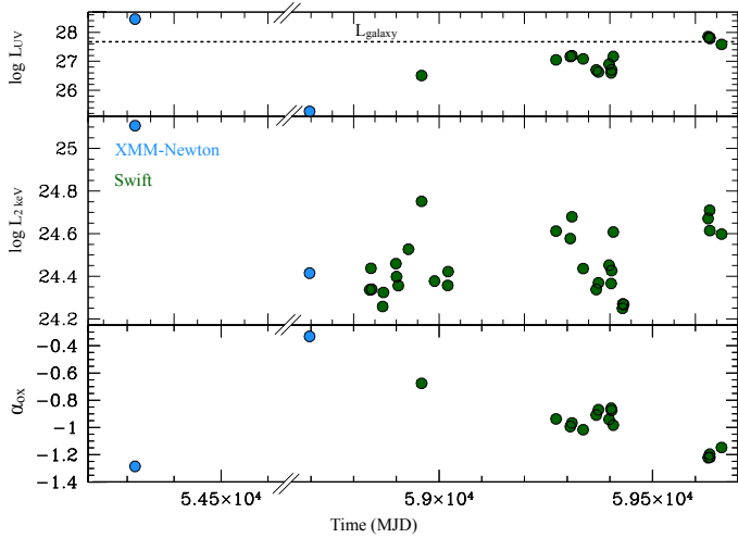
Fig. 12. Light curves for the AGN luminosity at 2500 \text{ \AA} , at 2 keV, and the inferred \alpha_{\text{OX}} . Blue dots identify values derived using XMM-Newton observations while in green the same quantities were estimated using Swift . The dashed horizontal line accounts for the adopted host galaxy luminosity at 2500 \text{ \AA} . Finally, both L_{\text{UV}} and L_{2 \text{ keV}} are in units of \text{erg s}^{-1} \text{ Hz}^{-1} .
