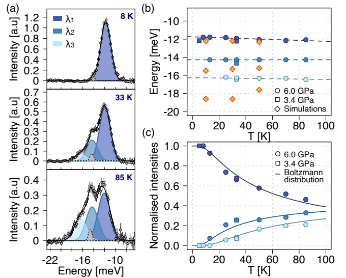
FIG. 4. Temperature dependence of the INS experimental results. (a): INS spectra at 6 GPa and 8 K, 33 K, 85 K, compared to their best fits (blue areas). The gray shaded area is the peak from the pure solid hydrogen in the sample. (b): Energies of the three rotational peaks at 6.0 and 3.4 GPa (blue circles and squares respectively) as a function of temperature compared with numerical results (yellow diamonds). (c): Normalised intensities of the three peaks at 6.0 and 3.4 GPa (blue circles and squares respectively) compared to the statistical weights of the initial states calculated using the Boltzmann distribution. Plots with error bars are reported in Fig. S14 in Supplementary Material [38]. The different blue shades are consistently associated to the transitions from the \lambda_1 , \lambda_2 , \lambda_3 levels to the ground state as shown in the legend.
