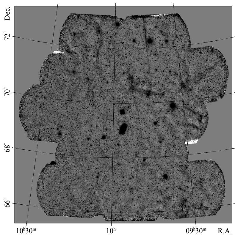
Figure 2. Mosaic image of M81 Group obtained through H\alpha filter. Image is displayed block averaged by 32 \times 32 pixels.
