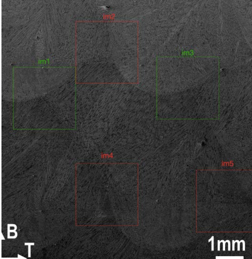
Figure 9: SEM image used as input to the CNN algorithm with the ZOIs indicated in green and red.
