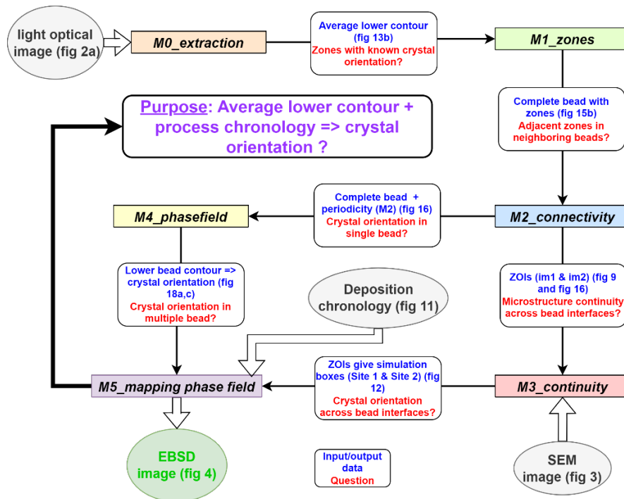
Figure 5 : Model layout. M0 to M5 indicate successive methods. The data transfers from one method to the next are indicated by dark arrows. Bold light grey arrows indicate experimental input.
