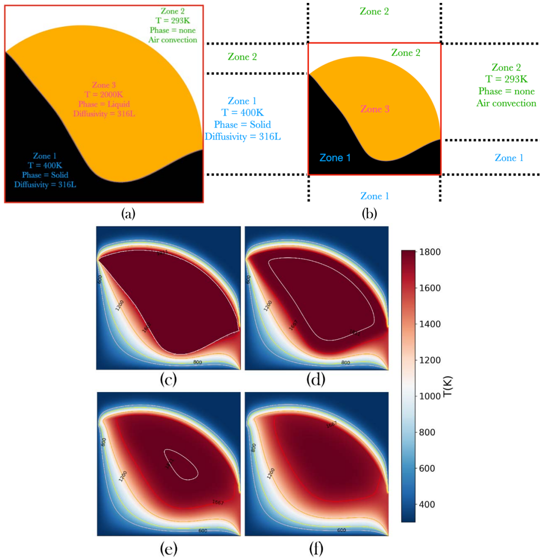
Figure 10 : Initial (a) and boundary conditions (b) as input for phase field simulation of bead solidification, (c) temperature field after respectively 60ms (c), 66ms (d), 72ms (e), 78ms (f).
