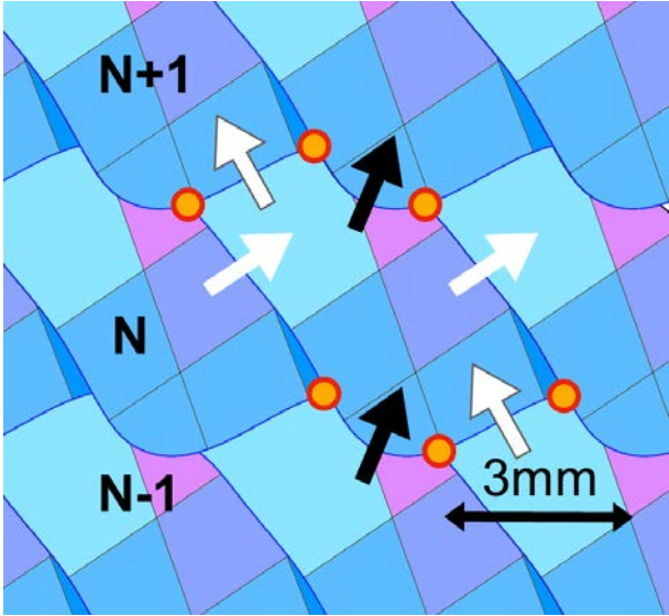
Figure 16 : Results of method M2. Mapping the entire plane with the flawless bead shape. Detection of possible continuity (white arrow and white arrow with black contour) or not (black arrow) crystal growth.
