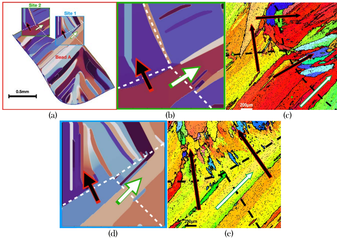
Figure 20 : Results of method M5. Check continuity of the microstructure. Positions of the ZOIs used for simulations (a), phase field simulation of continuity in Site 2 (b), zoom on in EBDS map (fig. 4) corresponding to location of Site 2 (c), phase field simulation at Site 1 (d), zoom on in EBDS map corresponding to location of Site 1 (e).
