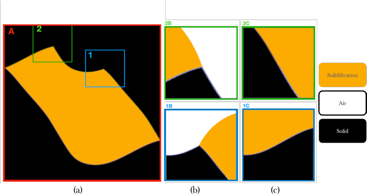
Figure 12 : Boundary and initial conditions applied to first and second simulation on Site 1 and Site 2.
