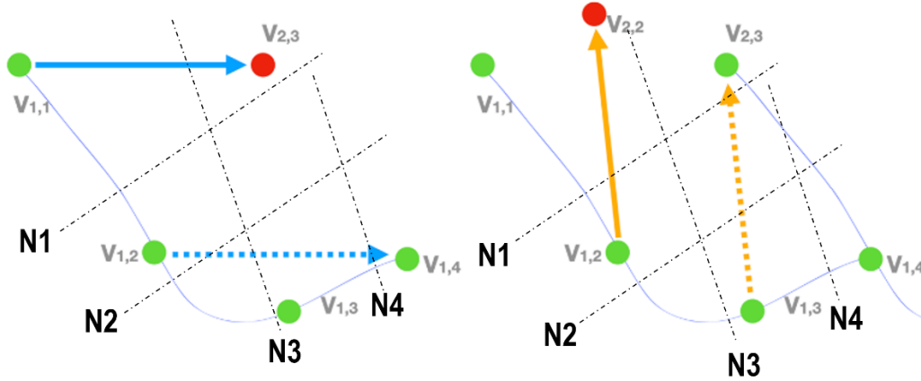
Figure 7: Method M1: At the beginning of the method vertices V_{1,i} (i=1, \dots, 4) are known. Vertices V_{2,2} and V_{2,3} are determined by M1 based on the periodicity at the bead scale.
