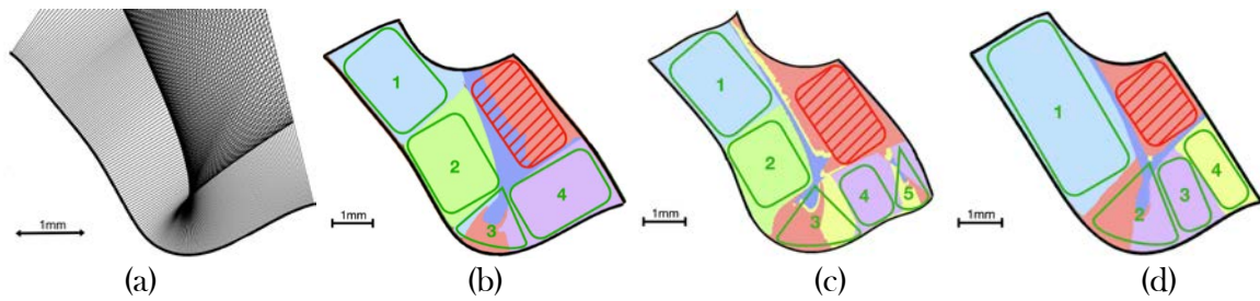
Figure 8 : Test results of CNN. The CNN was applied with the parameters given in tables 3 and 4 and as input, the images with the normals to the lower contour in (figures 14 a, b, c). Figure (a) shows the input used for the contour without defect. Figures (b-d) show results corresponding respectively to contours with defect to the left, no defect and a defect to the right. Different colors correspond to different zones detected by the CNN algorithm.
