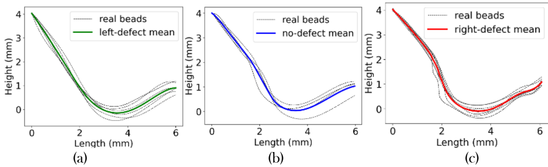
Figure 13 : Results of method M0. Typical bead shapes for the three types (defect to the left, without defect and defect to the right). Dashed lines represent different results obtained by segmentation. The thick colored lines represent the mean bead shape obtained as the mean value of the different cubic splines.
