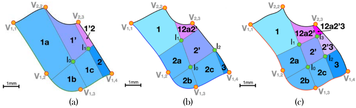
Figure 15 : Results of method M1. Predicted grain growth direction zones with defect on the left (a), without defect (b), with defect on the right (c)
