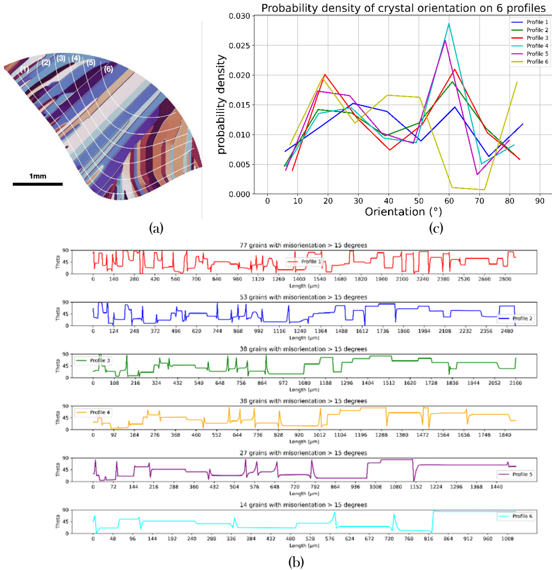
Figure 20 : Example analysis of phase field predictions ( M_5 ). profiles generated for the analysis (a), crystal orientation along each profile (b), histogram of crystal orientations for profiles (2) and (5), probability density of crystal orientation on all profiles (c).
