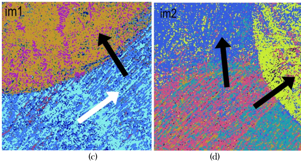
Figure 17: Results of method M3. Check continuity of the microstructure. (a) and (b) SEM ZOIs used as input to the CNN algorithm: im1 (a), im2 (b), with the ZOIs result corresponding to ZOI im1 and (c) result corresponding to ZOI im2 (d). White arrows indicate continuity of the microstructure, and black ones, discontinuity, i.e., different zones.
