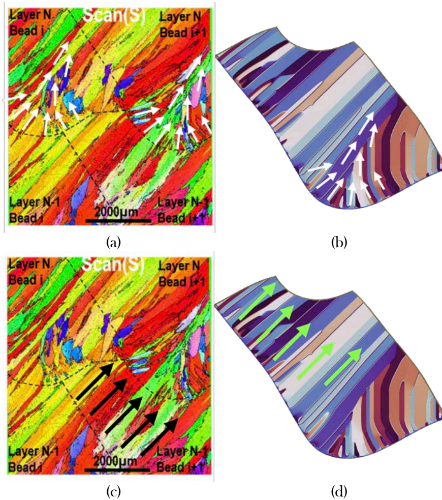
Figure 19 : Comparison between EBSD and simulation of crystal growth directions in the molten pool (a and b) and in the upper part of the beads (c and d).
