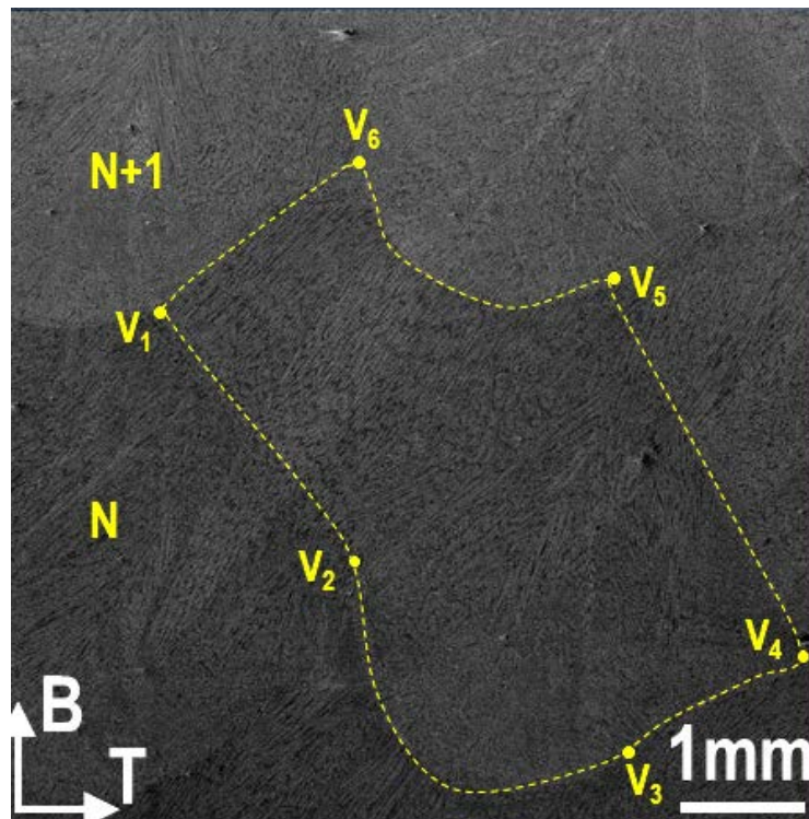
Figure 3 : SEM observation in a section perpendicular to the scanning direction. The light grey features correspond to \delta ferrite and the dark grey matrix corresponds to austenite. N and N+1 designate successive layers of material deposited. The yellow dashed line shows the border of a bead. V_i are vertices defining the bead. V_1 to V_4 are formed during deposition of layer N . V_5 and V_6 are formed during deposition of layer N+1 .
