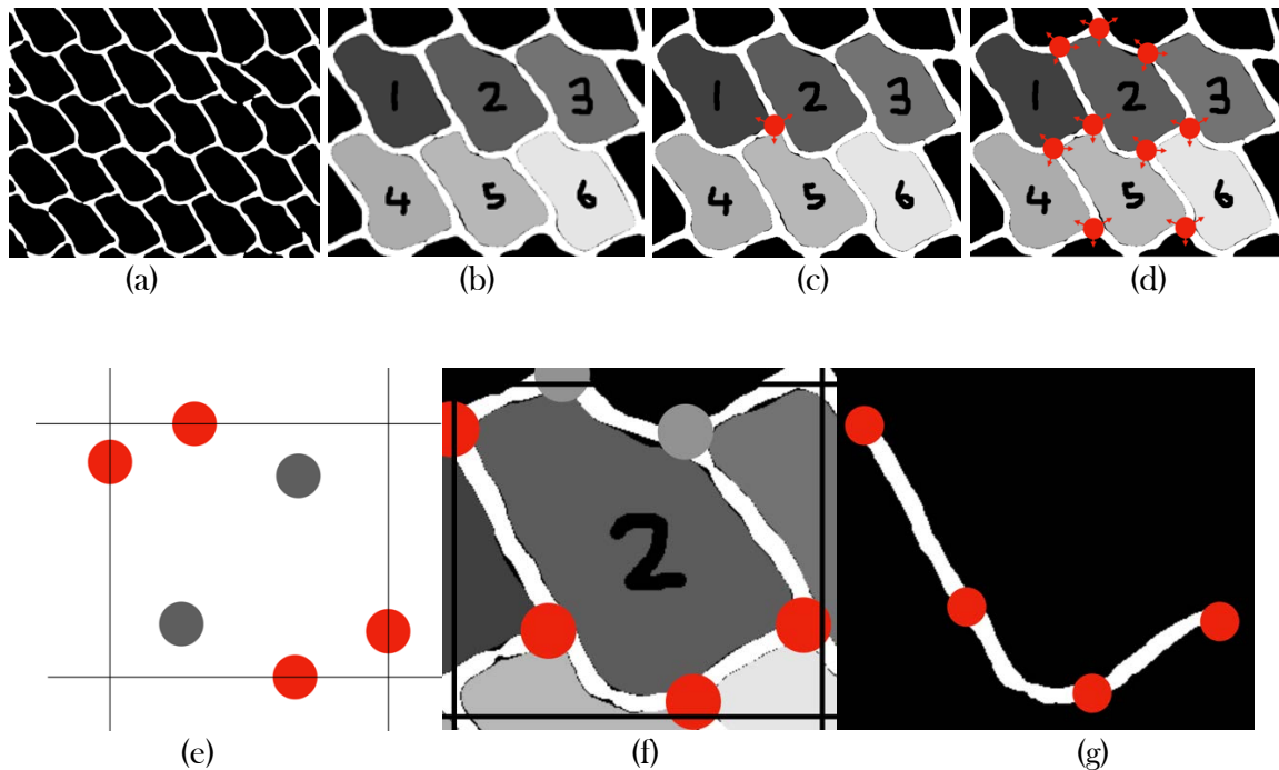
Figure 6: Detailed information for the set-up of method M0, the extraction of the lower bead contour.
