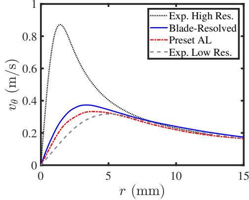
Figure 15: Tangential velocity around the tip vortex core.
