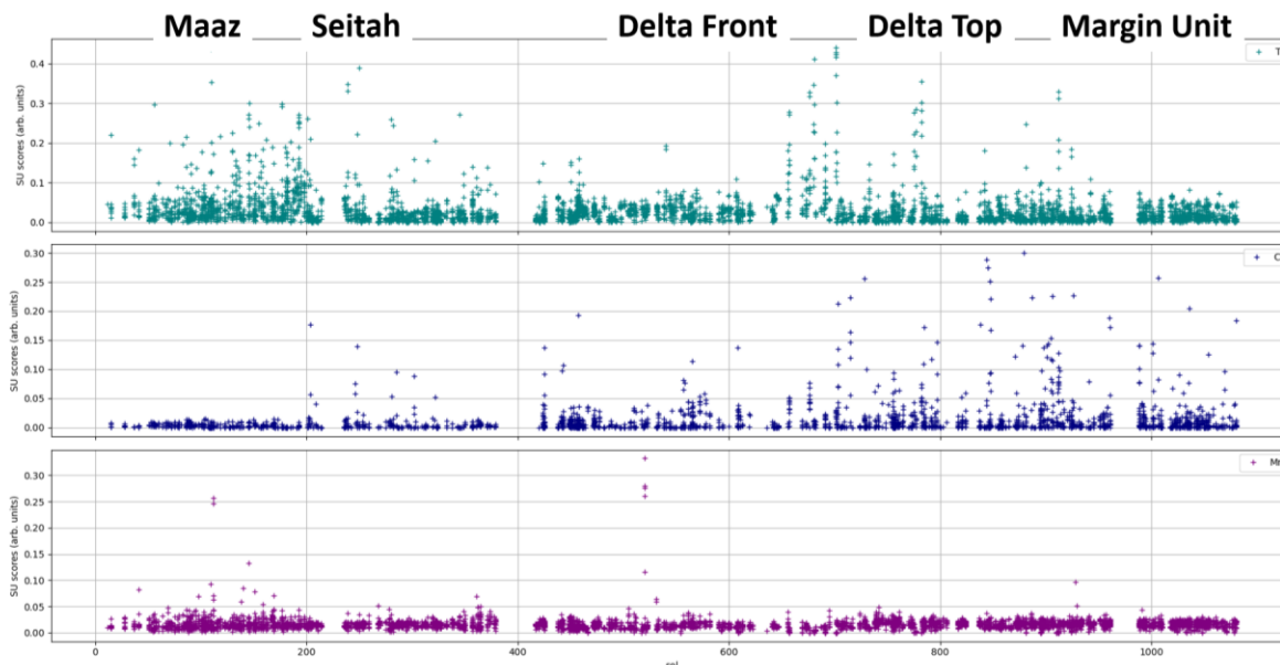
Figure 1: The spectral unmixing scores of (from top to bottom) Ti, Cr, and Mn with sol. Local variations and enrichments can be seen. Every element varies on their own scale so that the scores cannot be directly transferred into concentrations.
