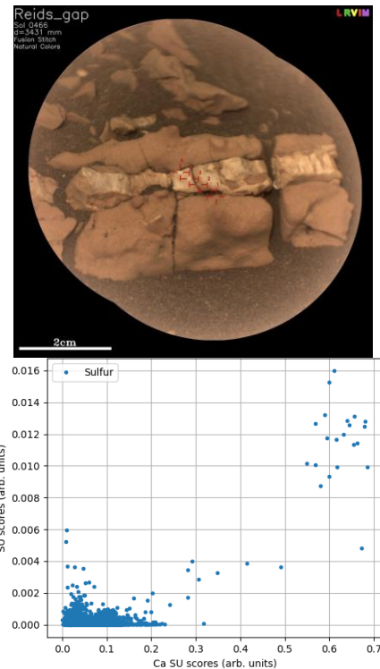
Figure 4: Calcium-sulfate veins such as the target Reids_gap (top) sampled on sol 466 at the delta front can be identified by their high S spectral unmixing score together with high Ca (bottom).
