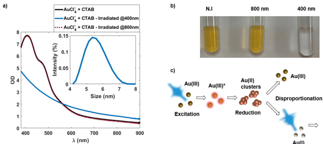
Figure 5: a) Absorption spectra of irradiated and unirradiated \text{AuCl}_4^- solutions without NR. Inset shows DLS sizing measurement for 400nm irradiation. b) Photographs of the \text{AuCl}_4^- solutions before and after irradiation at both wavelengths. c) Schematics of the proposed mechanism for \text{AuCl}_4^- photoreduction under 400 nm irradiation.
