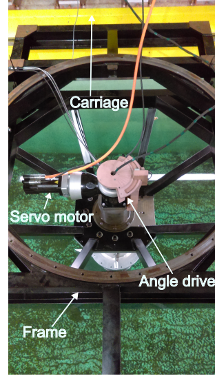
Figure 1: Top view of the experimental setup.
