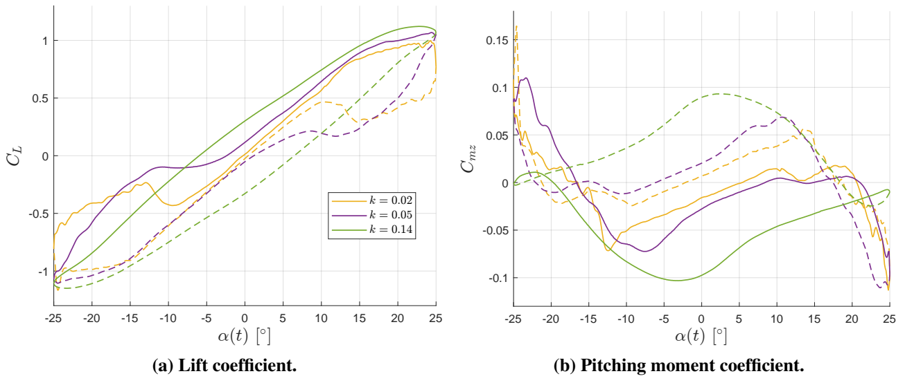
Figure 12: Dynamic hydrodynamic coefficients (various k , Re = 250\,000 , rigid hydrofoil).
