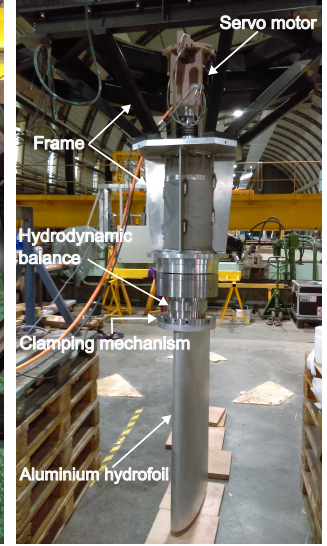
Figure 2: Out of water experimental setup, without hull.
