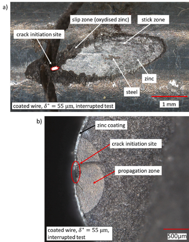
Fig. 15. Interrupted partial slip fretting fatigue test on coated wires, later broken with liquid nitrogen. P = 1400 \text{ N} , \sigma_m = 320 \text{ MPa} , \sigma_a = 160 \text{ MPa} , \delta^* = 55 \mu\text{m} , 70 000 cycles. a) Fretting scar at the end of the test, b) Longitudinal view.
