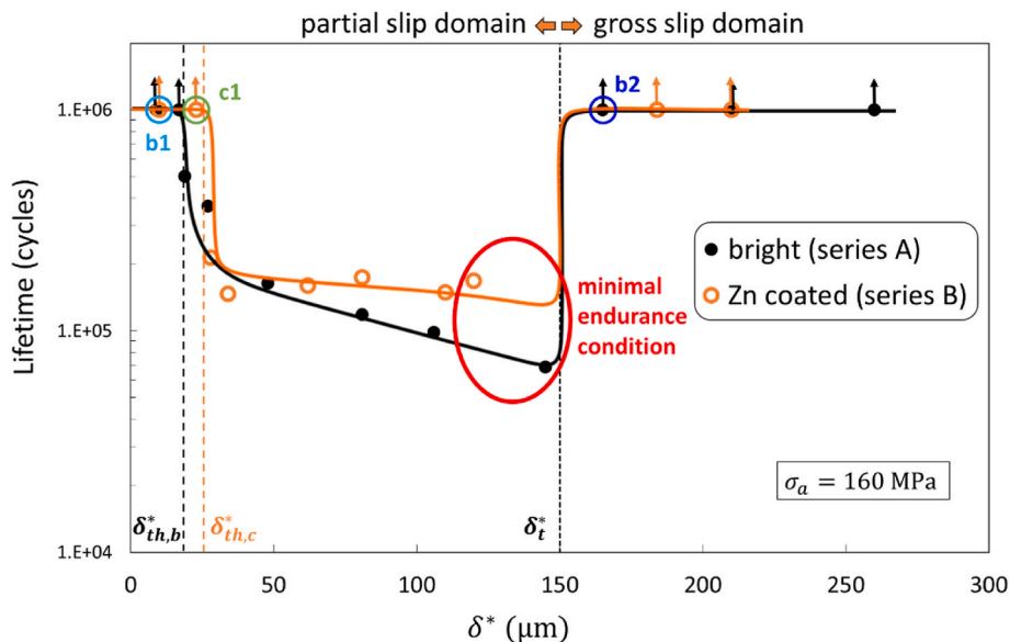
Fig. 5. Lifetimes of fretting fatigue tests on bright and zinc coated wires. Fixed fatigue load, varying fretting load. P = 1400 \text{ N} , \sigma_m = 320 \text{ MPa} , \sigma_a = 160 \text{ MPa} .
