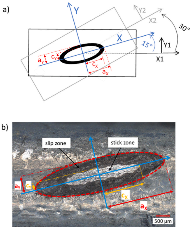
Fig. 4. a) Illustration of a fretting scar resulting from the crossed wires contact configuration, b) Fretting scar on a coated wire specimen after a partial slip fretting fatigue test.
