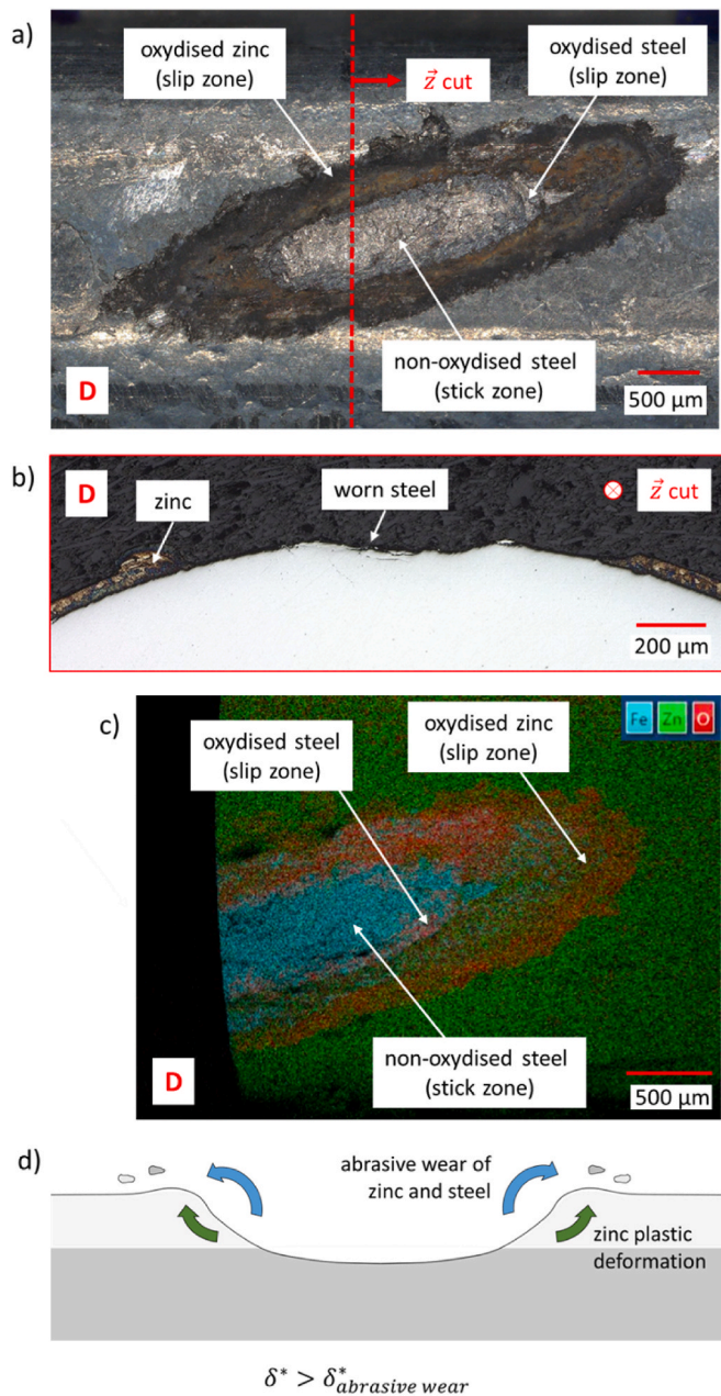
Fig. 20. Partial slip plain fretting test on coated wires “D” (indicated in Fig. 16). P = 1400 N, \delta^* = 185 \mu\text{m} , Q^* = 1350 N, 10 000 cycles. a) Optical view of the fretting scar at the end of the test, b) View of a transverse cross section of the wire, c) EDX view of the fretting scar for iron, zinc and oxygen elements. d) Illustration of the contact area extension mechanism for large displacement amplitudes.
