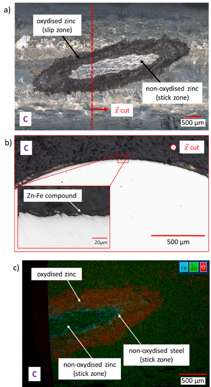
Fig. 19. Partial slip plain fretting test on coated wires “C” (indicated in Fig. 16). P = 1400\text{ N} , \delta^* = 80\ \mu\text{m} , Q^* = 550\text{ N} , 10 000 cycles. a) Optical view of the fretting scar at the end of the test, b) View of a transverse cross section of the wire, c) EDX view of the fretting scar for iron, zinc and oxygen elements.
