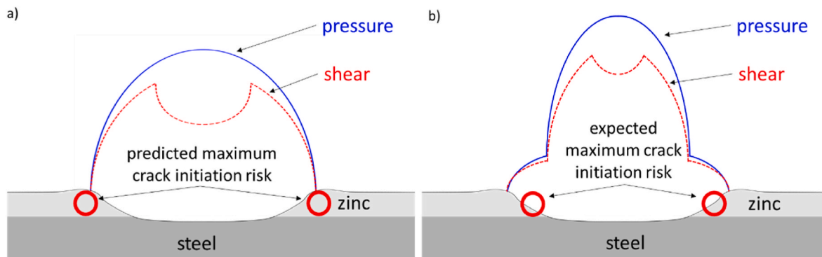
Fig. 21. Illustration of a) A classical distribution of pressure and shear profiles, used in the numerical model, and predicted maximum crack initiation risk, b) A composite description of expected pressure and shear considering the higher ductility of the Zn annulus, and expected maximum crack initiation risk.
