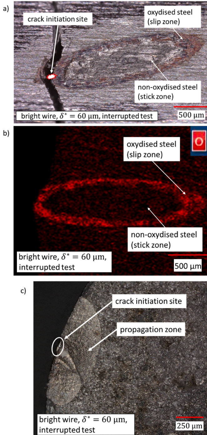
Fig. 12. Interrupted partial slip fretting fatigue test on bright wires, later broken with liquid nitrogen. P = 1400\text{ N} , \sigma_m = 320\text{ MPa} , \sigma_a = 160\text{ MPa} , \delta^* = 60\text{ }\mu\text{m} , 70 000 cycles. a) Optical view of the fretting scar at the end of the test, b) EDX view of the fretting scar at the end of the test for oxygen element, c) Longitudinal view.
