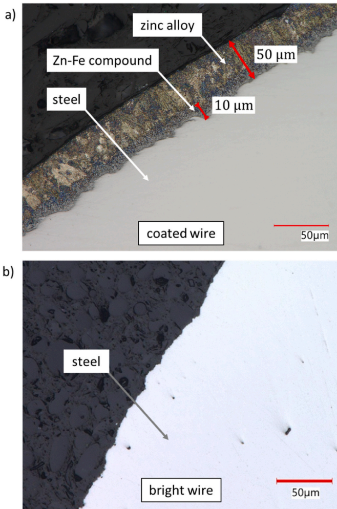
Fig. 1. a) Transverse section of a coated wire, b) Transverse section of a bright wire, after removal of the coating.
