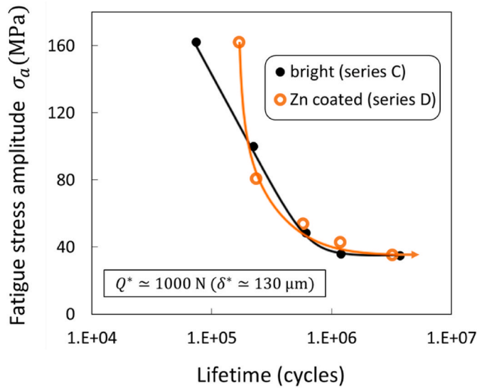
Fig. 9. Lifetimes of fretting fatigue tests on bright and zinc coated wires. Fixed fretting load, varying fatigue load. P = 1400 \text{ N} , \sigma_m = 320 \text{ MPa} , Q^* \approx 1000 \text{ N} ( \delta^* \approx 130 \text{ }\mu\text{m} ).
