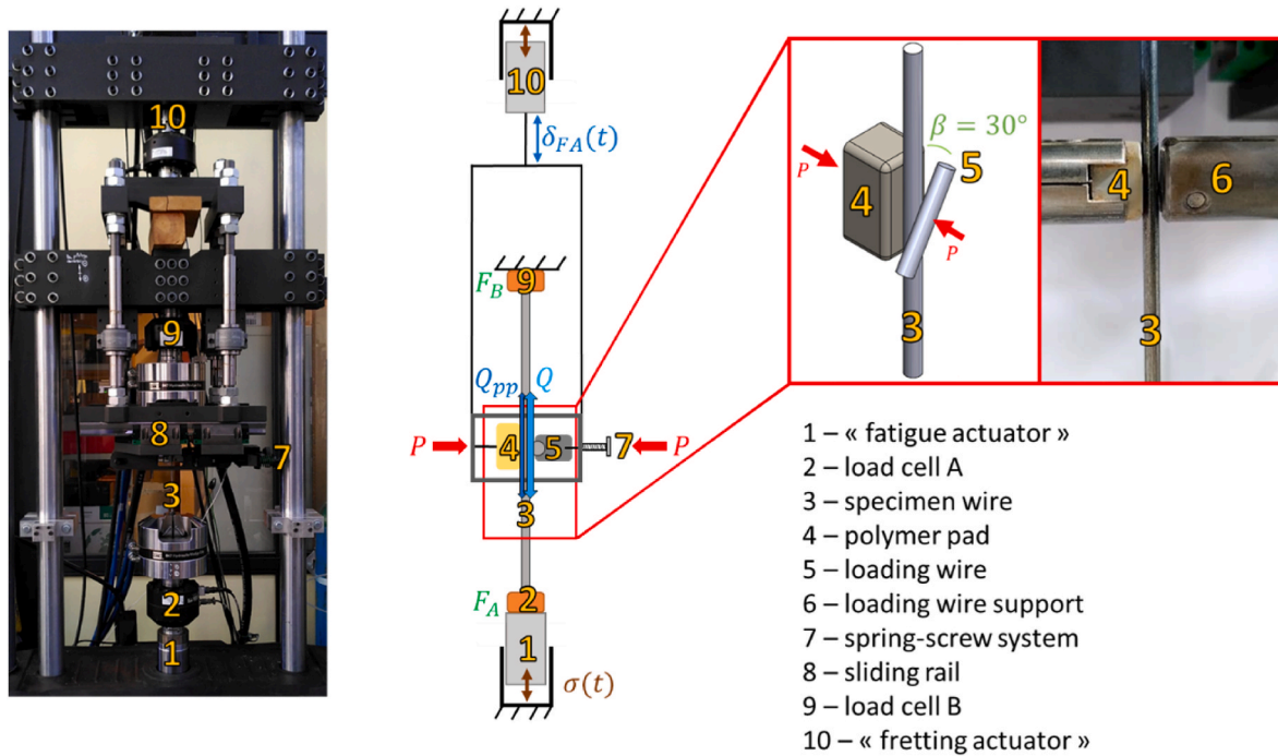
Fig. 2. Fretting fatigue test rig.
