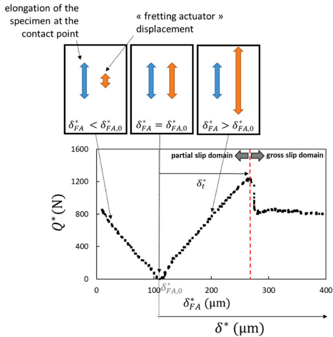
Fig. 3. Illustrated variable displacement test on bright wires with fatigue load. P = 1400\text{ N} , \sigma_m = 320\text{ MPa} , \sigma_a = 160\text{ MPa} .
