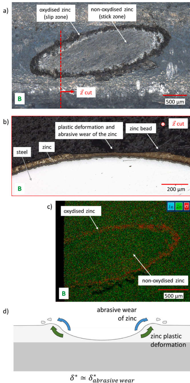
Fig. 18. Partial slip plain fretting test on coated wires “B” (indicated in Fig. 16). P = 1400\text{ N} , \delta^* = 50\ \mu\text{m} , Q^* = 400\text{ N} , 10 000 cycles. a) Optical view of the fretting scar at the end of the test, b) View of a transverse cut of the wire, c) EDX view of the fretting scar for iron, zinc and oxygen elements. d) Illustration of the contact area extension mechanism for intermediate displacement amplitudes.
