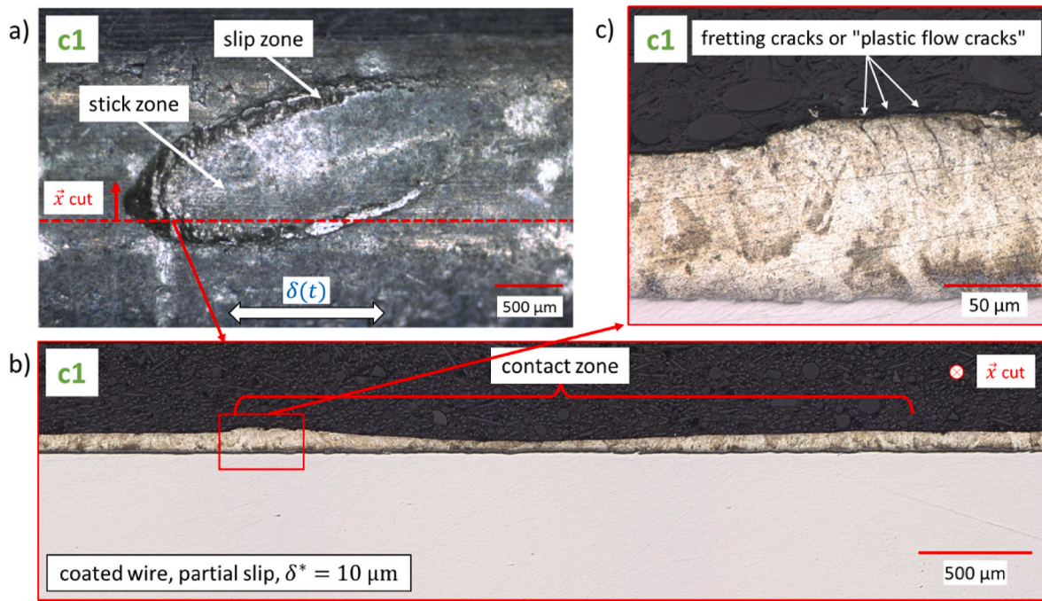
Fig. 14. Partial slip fretting fatigue test on coated wires “c1” (indicated in Fig. 5) P = 1400 \text{ N} , \sigma_m = 320 \text{ MPa} , \sigma_a = 160 \text{ MPa} , \delta^* = 10 \mu\text{m} . a) Fretting scar at the end of the test, b,c) Views of a longitudinal cut of the wire.
