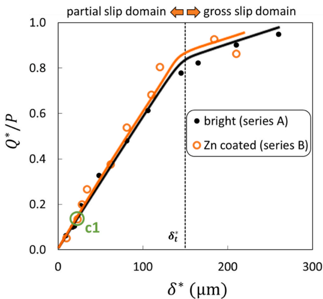
Fig. 7. Normalized tangential force amplitudes of fretting fatigue tests on bright and zinc coated wires. Fixed fatigue load, varying fretting load. P = 1400 \text{ N} , \sigma_m = 320 \text{ MPa} , \sigma_a = 160 \text{ MPa} .
