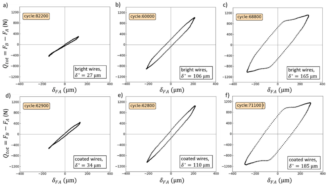
Fig. 6. Fretting loops for several fretting fatigue tests on bright and coated wires displayed in Fig. 5. P = 1400 \text{ N} , \sigma_m = 320 \text{ MPa} , \sigma_a = 160 \text{ MPa} .
