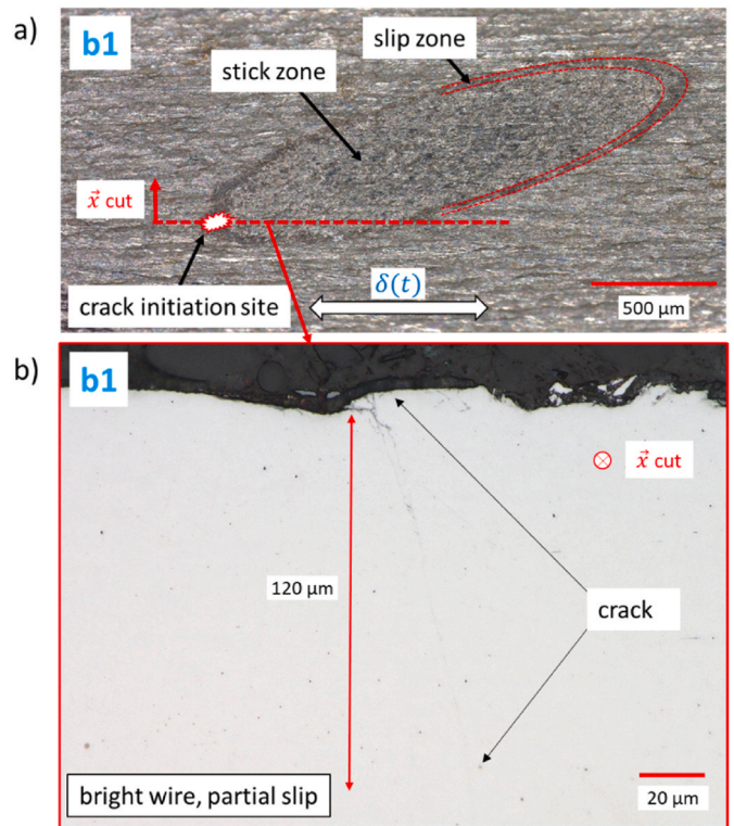
Fig. 11. Partial slip fretting fatigue test on bright wires “b1” (indicated in Fig. 5) P = 1400 \text{ N} , \sigma_m = 320 \text{ MPa} , \sigma_a = 160 \text{ MPa} , \delta^* = 10 \text{ }\mu\text{m} . a) Fretting scar at the end of the test, b) Longitudinal cross section of the wire.
