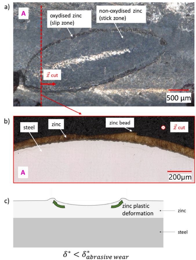
Fig. 17. Partial slip plain fretting test on coated wires "A" (Fig. 16). P = 1400 N, \delta^* = 20 \mu\text{m} , Q^* = 130 N, 10^4 cycles. a) Fretting scar at the end of the test, b) View of a transverse cross section of the wire. c) Illustration of the contact area extension mechanism for low displacement amplitudes.
