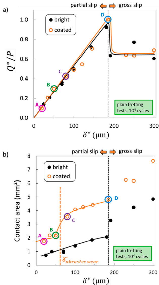
Fig. 16. Plain fretting tests on bright wires and coated wires. P = 1400 N, 10^4 cycles. a) Normalized tangential force amplitude means, b) Contact areas at the end of the tests, in function of effective displacement amplitudes.
