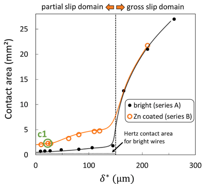
Fig. 8. Contact areas at the end of fretting fatigue tests on bright and zinc coated wires. Fixed fatigue load, varying fretting load. P = 1400 \text{ N} , \sigma_m = 320 \text{ MPa} , \sigma_a = 160 \text{ MPa} .
