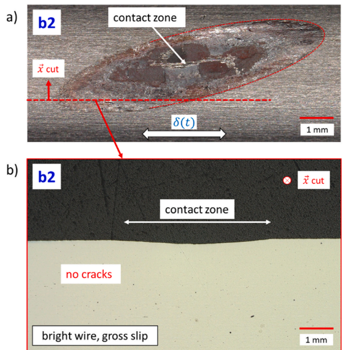
Fig. 13. Gross slip fretting fatigue test on bright wires “b2” (indicated in Fig. 5). P = 1400\text{ N} , \sigma_m = 320\text{ MPa} , \sigma_a = 160\text{ MPa} , \delta^* = 210\text{ }\mu\text{m} . a) Fretting scar at the end of the test, b) Longitudinal cross section of the wire.
