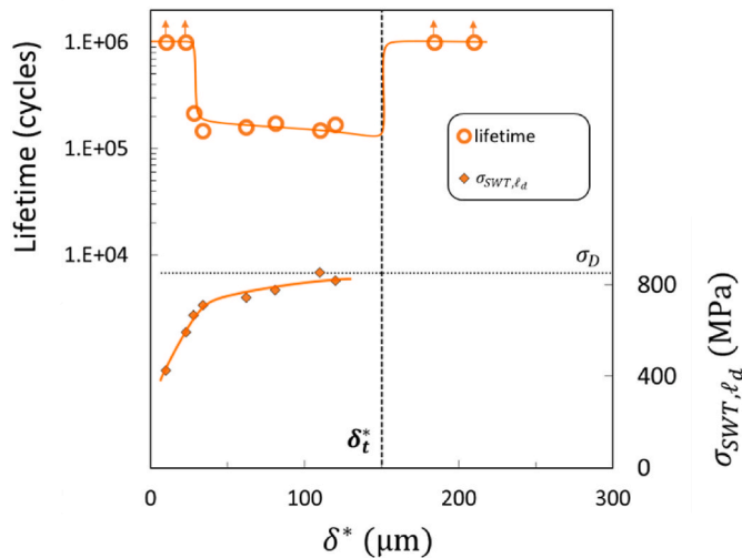
Fig. 10. Experimental lifetimes and numerically calculated \sigma_{SWT,ld} for fretting fatigue tests of series B (coated wires).
