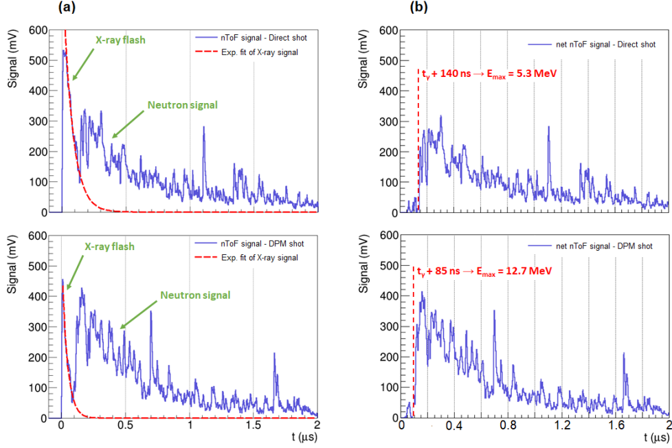
Fig. 11 (a) nToF signals obtained with the scintillator #16 placed at 4.95 m from TCC and at 19° from the normal axis. These signals were acquired during a direct shot with a 1.5 \mu\text{m} Al target (top) and a DPM shot with a 200 nm Si + 50 nm Al target (bottom). The exponential fits of the X-ray signals used for the background noise subtraction are shown in red dashed lines. (b) Net neutron signals obtained after removal of the signal induced by the X-rays. The red dashed lines correspond to the ToF of the most energetic neutrons detected.
