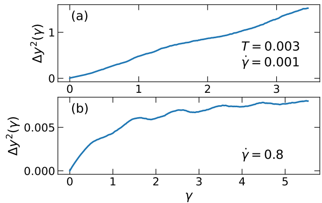
FIG. 9. Mean square displacement \Delta y^2(\gamma) along the direction perpendicular to the shear for one trajectory in the steady state as a function of the strain \gamma for two different shear rates, \dot{\gamma} = 10^{-3} (a) and \dot{\gamma} = 0.8 (b), at a temperature T = 0.0030 . \gamma is measured from a configuration in the steady state. The top panel corresponds to Regime I and the bottom one to Regime III.
