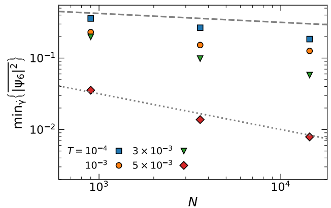
FIG. 13. System-size dependence of \min_{\dot{\gamma}} \{|\psi_6|^2\} , the minimum value over \dot{\gamma} reached by |\psi_6|^2 in Fig. 4(a), for various temperatures below the putative T_{m,\text{sol}} . The dashed and dotted lines indicates a L^{-1/4} and a L^{-1} dependence, respectively.
