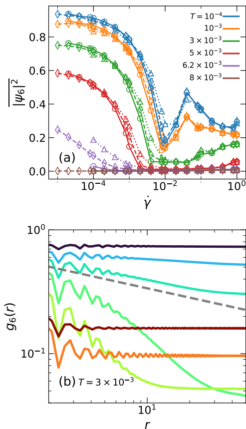
FIG. 4. (a): Averaged square modulus of the bond-orientational order parameter, |\overline{\psi_6}|^2 , as a function of shear rate for various temperatures and system sizes. Triangles (with dotted-line), diamonds (dashed-line), and circles (solid-line) correspond to data for N = 900 , 3600 , and 14400 , respectively. (b): Spatial decay of the bond-orientational correlation function g_6(r) for T = 0.0030 , N = 14400 , and a wide range of \dot{\gamma} . The grey dashed line represents the bound imposed on a power-law decay by the KTHNY theory, g_6(r) \sim r^{-1/4} .
