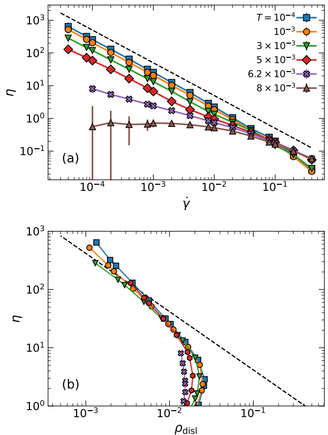
FIG. 3. (a): Log-log plot of the effective viscosity \eta = \bar{\sigma}/\dot{\gamma} as a function of the shear rate \dot{\gamma} for the same data as in Fig. 2(a). The dashed straight line shows the dependence \eta \sim \dot{\gamma}^{-1} . (b): Log-log plot of the effective viscosity as a function of the density of dislocations \rho_{\text{disl}} . The dashed line corresponds to \eta \sim \rho_{\text{disl}}^{-1} .
