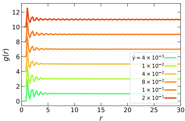
FIG. 10. Radial distribution function g(r) for a system of N = 14400 particles at a temperature T = 0.0030 and for several shear rates \dot{\gamma} covering the three regimes of flow. The data for different \dot{\gamma} are shifted along the y -axis for clarity.
