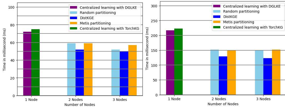
Fig. 2 Results of training time on the FB15K dataset Fig. 3 Results of training time on the MalKG dataset
