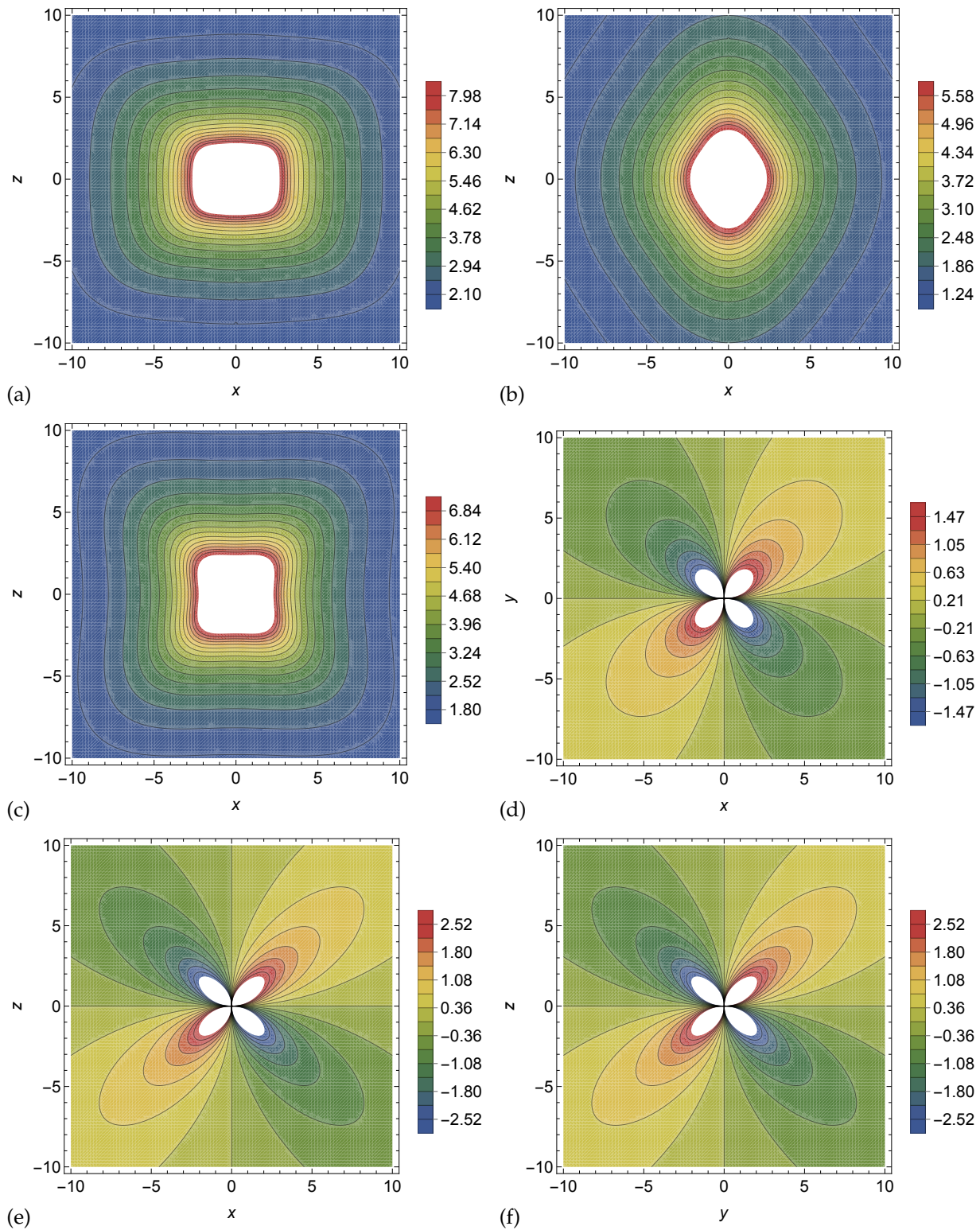
Figure 1. Phonon components of the Green tensor: (a) G_{11}^{\parallel\parallel} \times 10^4 , (b) G_{22}^{\parallel\parallel} \times 10^4 , (c) G_{33}^{\parallel\parallel} \times 10^4 , (d) G_{12}^{\parallel\parallel} \times 10^4 , (e) G_{13}^{\parallel\parallel} \times 10^4 , (f) G_{23}^{\parallel\parallel} \times 10^4 .
