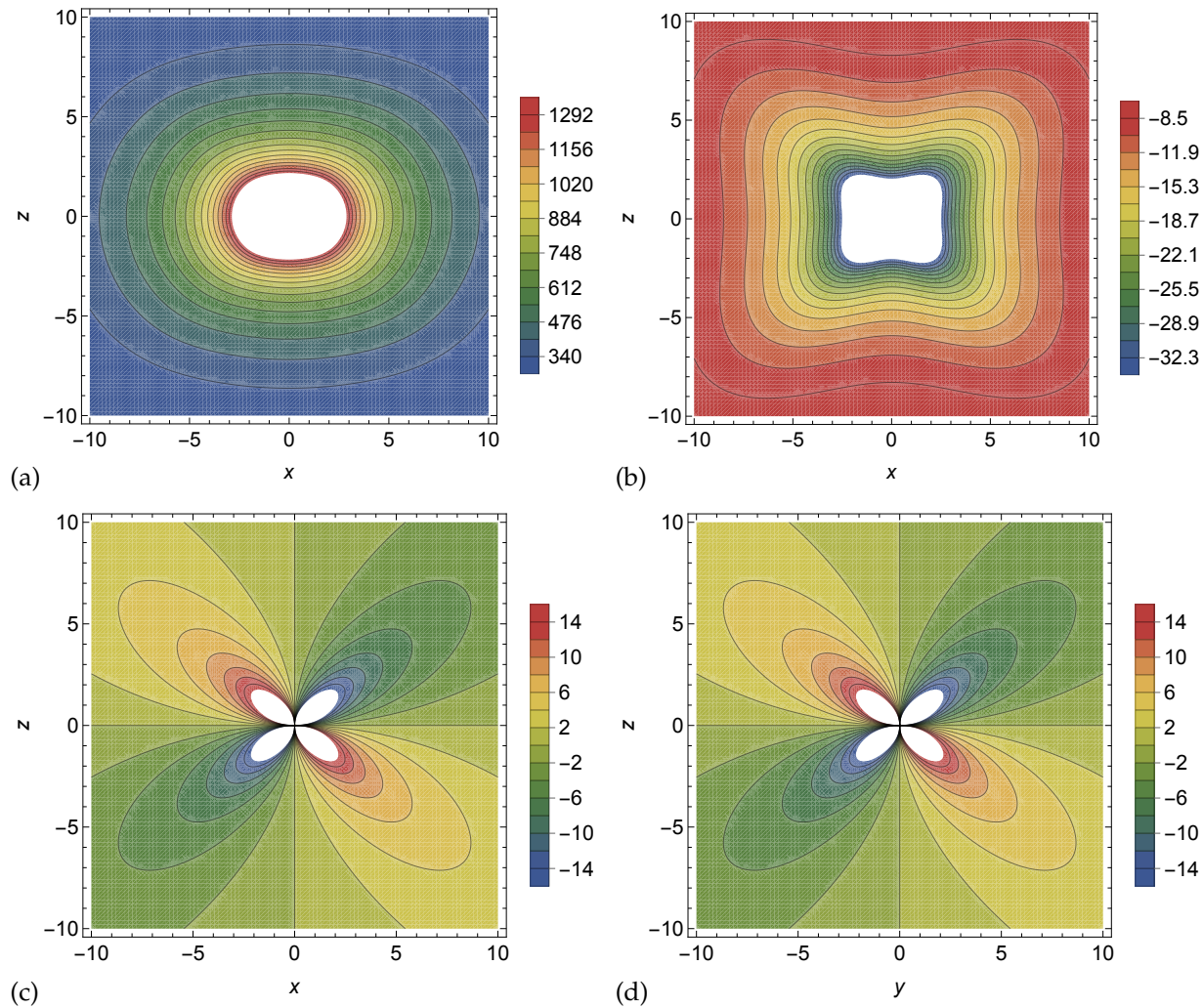
Figure 2. Phason and phonon-phason coupling components of the Green tensor: (a) G_{44}^{\perp\perp} \times 10^4 , (b) G_{34}^{\parallel\perp} \times 10^4 , (c) G_{14}^{\parallel\perp} \times 10^4 , (d) G_{24}^{\parallel\perp} \times 10^4 .
