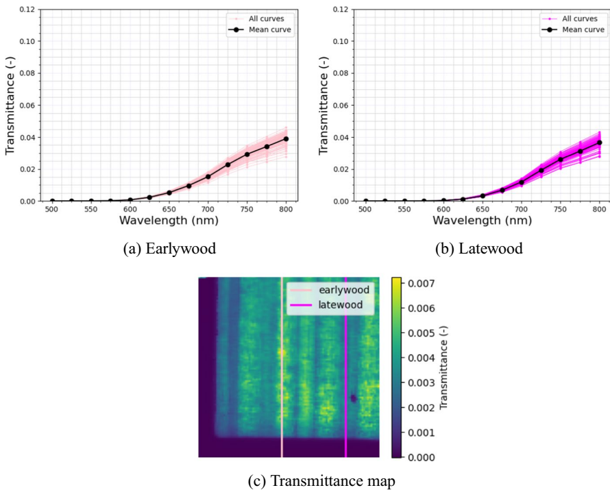
Fig. 11 Transmittance ( T_{r,wood} ) evolution for one line of a earlywood, b latewood, c transmittance map
