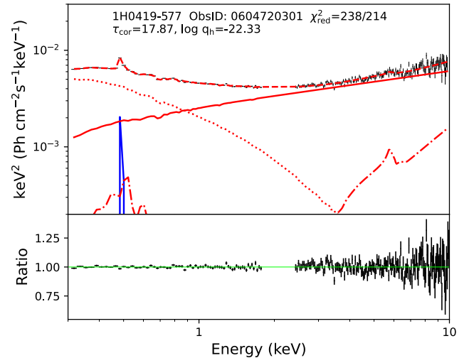
Fig. C.1. Example of an unfolded best-fit model of 1H0419-577 (ObsID: 0604720301) using relativistic reflection model and its data/model ratio, as described in Appendix C. The data are in black crosses. RELXILL model is represented by dashed-dotted line, NTHCOMP by solid line and TITAN-NOAR by a dotted line. A narrow Gaussian at 0.537 keV is shown as a blue solid line.
