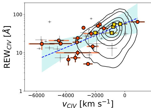
Fig. 3. The REW_{CIV} vs. v_{CIV} relation compared with the 0.05, 0.1, 0.3, 0.5, 0.68, 0.9 and 0.99 contour levels (relative to the peak) of the SDSS DR7 sample (Shen et al. 2011; Vietri et al. 2018) and with the values from Schindler et al. 2020 (grey points). For simplicity, we plot here the mean values derived using all the available values reported in Table 3. We note that the fit takes into account all the existing values of v_{CIV} and REW_{CIV} (see Section 3.2).
