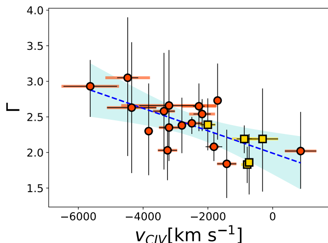
Fig. 1. Plot of \Gamma vs. v_{CIV} . The orange circles and the yellow squares represent the HYPERION and non-HYPERION QSOs, respectively. For simplicity we report in the plot the mean values of v_{CIV} (see Table 1), but the fit takes into account all the existing values of v_{CIV} (see Section 3.2). The thick coloured errorbars represent the maximum deviation from the mean, while the thin black errorbars represent the mean error. The dashed blue line is the linear regression while the shaded region represents the combined 1\sigma error on the slope and normalization (see Table 5). This is valid for all the following plots.
