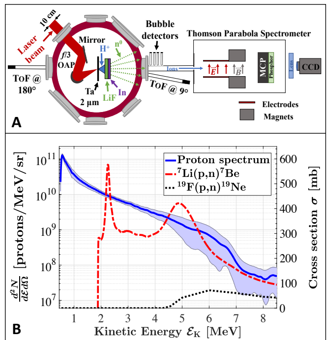
FIG. 1. (A) Top-view of the experimental setup for the laser-driven neutron generation. (B) Mean proton spectrum averaged over 38 shots using a 2 \mu\text{m} -thick tantalum foil (full blue). The shaded area is delimited by one standard deviation. The cross sections for the nuclear reactions {}^7\text{Li}(p,n){}^7\text{Be} (dashed red) and {}^{19}\text{F}(p,n){}^{19}\text{Ne} (dotted black) are also shown, as given by the ENDF/B-VIII.0 34 and TENDL-2019 libraries 35 , respectively.
