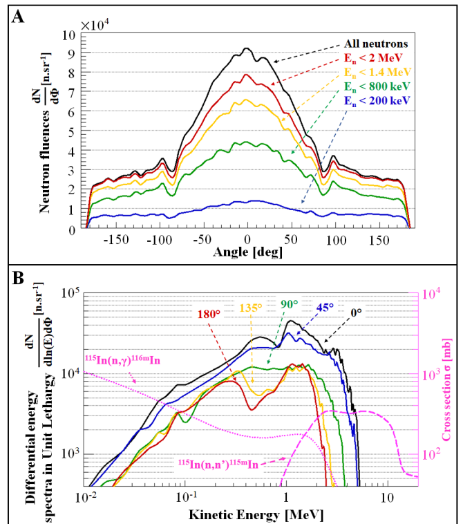
FIG. 2. (A) Simulated angular distribution of the neutron emissions recorded in the equatorial plane and passing through the converter center, and (B) differential energy spectra, in unit lethargy, obtained at different angles from Geant4 simulations. Overlaid are the cross sections (in pink) of the {}^{115}\text{In}(n, \gamma){}^{116\text{m}}\text{In} and {}^{115}\text{In}(n, n'){}^{115\text{m}}\text{In} reactions, according to the IRDFF-II 40 library. These are used for the activation simulations.
