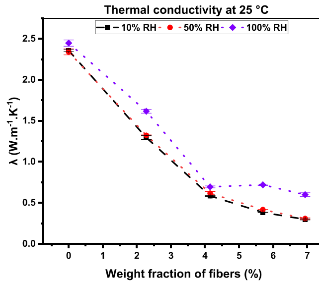
Fig. 12. Dependence of the thermal conductivity of mortars at 25°C upon the weight content of miscanthus fibers, for different levels of relative humidity.
