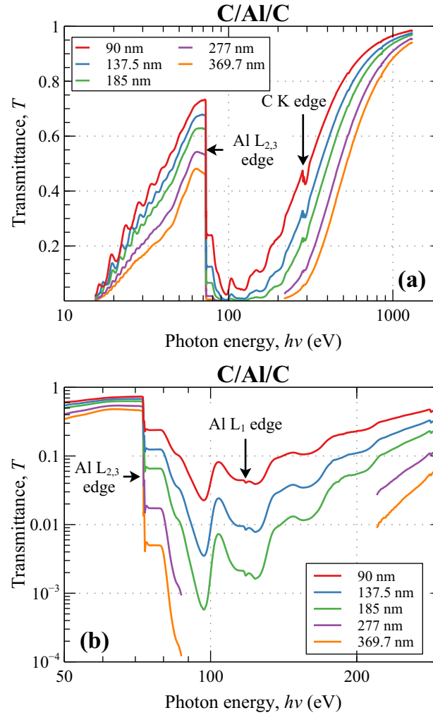
FIG. 3. Experimental transmittance vs. photon energy spectra for all C/Al/C samples: (a) log-linear plot, (b) log-log plot focused in the photon energy range 50 – 300 eV.
