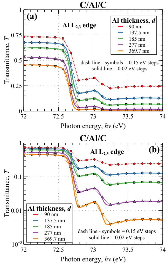
FIG. 4. Experimental transmittance vs. photon energy spectra for C/Al/C samples in the vicinity of the Al L_{2,3} edge: (a) lin-lin plot and (b) lin-log plot. Measurements with larger photon energy step size (0.15 eV steps) were performed initially and are shown as a dash line and symbols. Measurements with ultra-low step size (0.02 eV steps) were performed later and are shown as a solid line.
