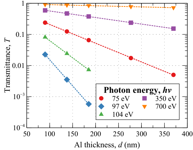
FIG. 5. Transmittance (log axis) vs. Al thickness (linear axis) for various photon energies. The symbols show the measured transmittance data and the dashed lines represent the fit to the data, according to eq. (2).
