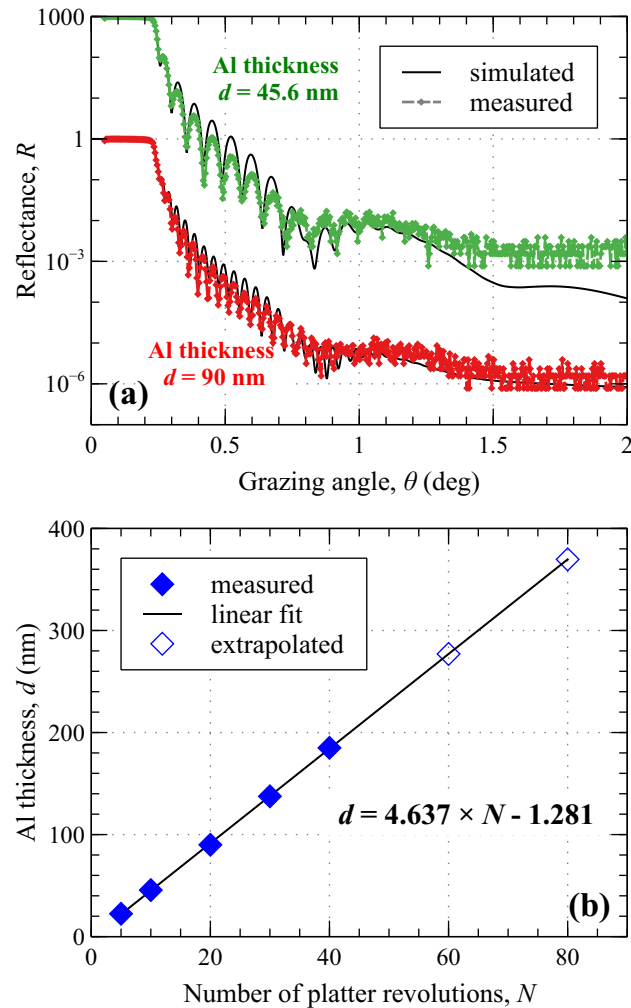
FIG. 1. (a) GIXR data of two C/Al/C films deposited on a Si wafer. The measured data are shown in green and red dots and the simulated curves are shown as black solid lines. The thicknesses of the Al layers, simulated to fit the GIXR data, are 45.6 nm (green) and 90 nm (red), and the C layers are 5.5 nm thick each. The plots from the 45.6 nm thick Al film have been shifted on the y-axis, for better visibility (b) Measured Al thickness (blue filled diamonds) and linear fit (black line) as a function of the number of platter revolutions. The Al thicknesses were obtained by fitting the GIXR data, as illustrated in (a). The linear fit was used to extrapolate the thickness values for the two thickest films (blue unfilled diamonds).
