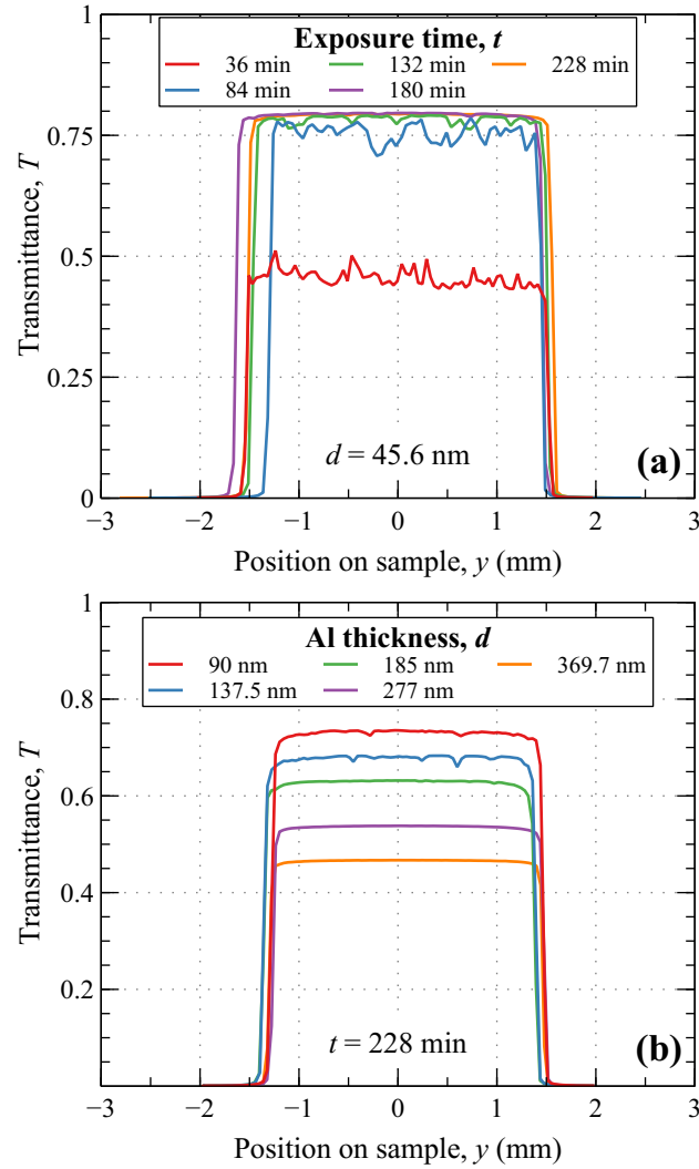
FIG. 2. Measured transmittance at 70.85 eV, as a function of the vertical position on the sample, on (a) a C/Al/C film with an Al thickness of 45.6 nm, for various exposure times to the UV-ozone lamp, and (b) all C/Al/C samples used in the present study (with the Al thickness shown in the legend), with an exposure time of 228 min.
