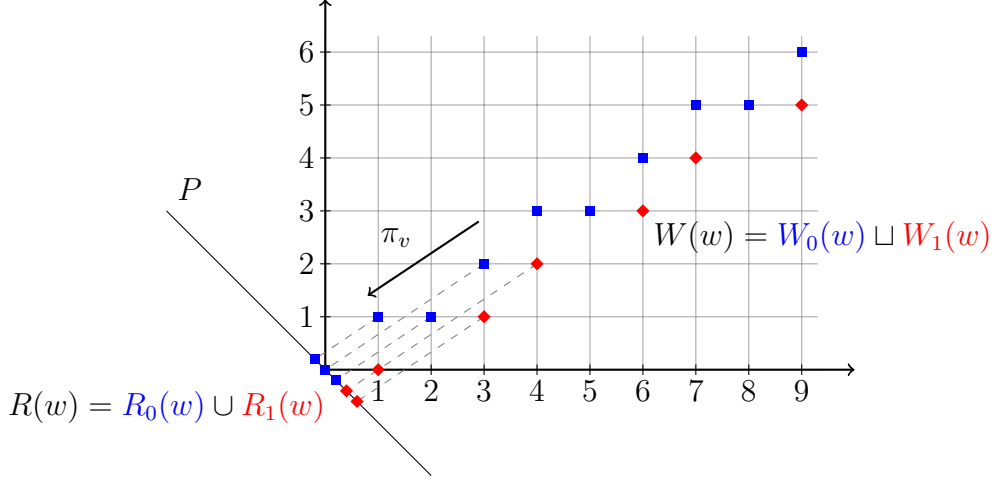
Figure 5: The Rauzy fractal R(w) as the closure of the projection of the worm W(w) on the hyperplane P . Example for w = (01001)^\omega , so v = (3/5, 2/5) .
