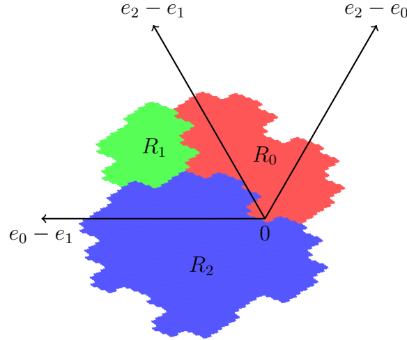
Figure 6: Approximation of the Rauzy fractal of a directive sequence beginning with c_1 c_1 c_0 c_1 c_0 c_0 c_0 c_1 c_1 c_1 c_0 c_1 c_0 c_0 c_1 c_0 c_1 c_0 c_0 c_0 c_1 c_0 c_1 c_1 c_1 c_0 c_1 c_1 c_1 c_0 c_0 c_1 c_0 c_0 c_0 c_1 c_1 c_0 c_0 c_0 , where c_0 and c_1 are defined in Section 8.
