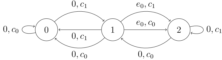
Figure 11: Abelianized prefix automaton for S = \{c_0, c_1\} .
