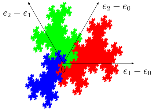
Figure 8: Rauzy fractal of the directive sequence (b_{210}b_{021}b_{102})^\omega .
