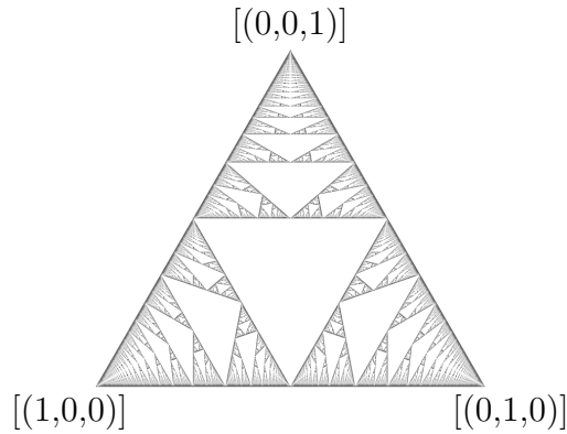
Figure 9: The Rauzy gasket X \subseteq \mathbb{P}\mathbb{R}_+^2 .
