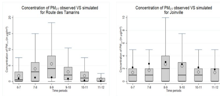
The PM_{2.5} observed concentrations at the air pollution station Route des Tamarins during the morning peak, which is the time period from 6 a.m. to 12 p.m., are shown using boxplots in the left figure. Our predicted concentrations at the station's location are represented by the black dots. For our baseline parametrization, they are computed using our Gaussian plume model, in which we integrated the outcomes of our emissions model. The identical outcomes are shown in the right figure, but for the Joinville air pollution station. Source: AtmoRéunion, 2019
