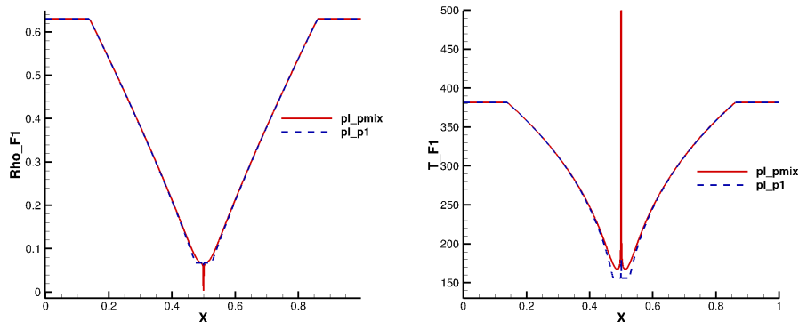
Figure 2: Gas density (left) and gas temperature (right) for the double rarefaction Riemann problem.
