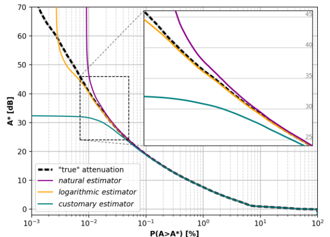
Fig. 12. CCDFs of excess attenuation from the noiseless synthetic time series (ideal receiver) generated using ITU-R P.1853, and from the three estimators in presence of thermal noise (actual receiver).
