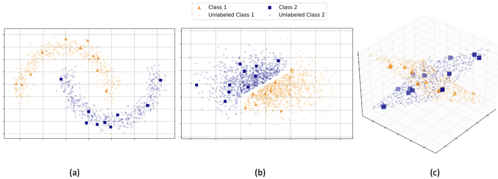
Figure 1: Illustration of three main hypotheses made in semi-supervised learning: (a) cluster assumption, (b) low-density separation and (c) manifold assumption.
