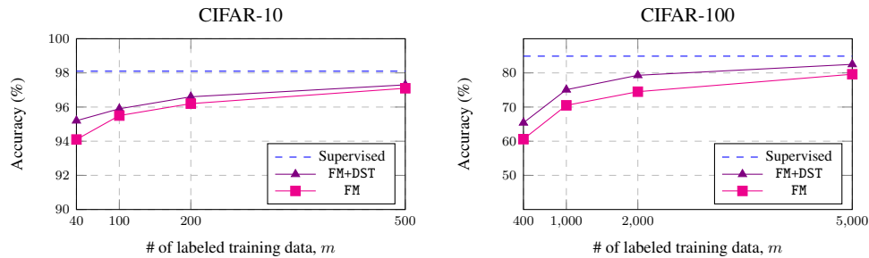
Figure A.2: Comparisons in terms of Accuracy on CIFAR-10 and CIFAR-100 for a varying number of labeled training data. “Supervised” refers to the fully supervised learning ( m = 50000, u = 0 ).
