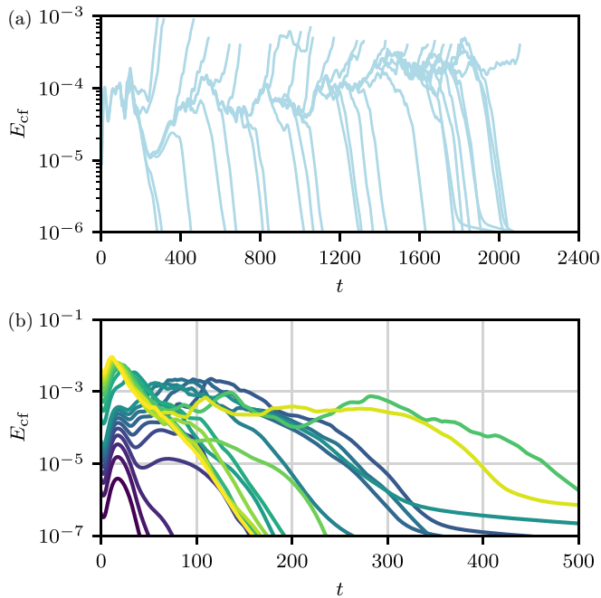
FIG. 16. Time series of E_{cf}(t) beyond the tipping point for Ha = 20 . (a) Trajectories reaching the predefined (but repeatedly readjusted) threshold levels E^{\text{turb}} and E^{\text{lam}} . (b) Trajectories with initial perturbation amplitudes A in (B2) logarithmically distributed between 10^{-3} (dark blue) and 10^{-1} (yellow). All trajectories eventually laminarize without reaching any equilibrium level, making it impossible to define a turbulent level and hence to select an edge trajectory in (a).
