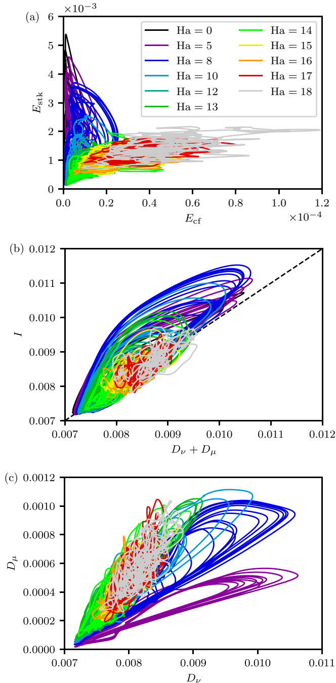
FIG. 6. State portraits of the edge state for different Ha. (a) Cross-flow energy ( E_{\text{cf}} ) plotted against streak energy ( E_{\text{stk}} ). (b) Energy input ( I ) plotted against total dissipation ( D_v + D_\mu ). (c) Joule dissipation ( D_\mu ) plotted against viscous dissipation ( D_v ). The color coding is the same for all state portraits.
