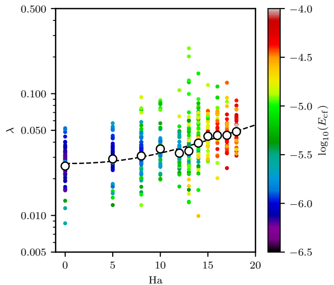
FIG. 11. Finite-size Lyapunov exponent \lambda as a function of \text{Ha} (open circles), and its fluctuations (colored dots). The dots are colored according to the instantaneous cross-flow energy E_{cf} of the edge states. The dashed line is a power-law fit of the form c + b\text{Ha}^a with a = 2.31 , b = 2.86 \times 10^{-5} and c = 2.67 \times 10^{-2} .
