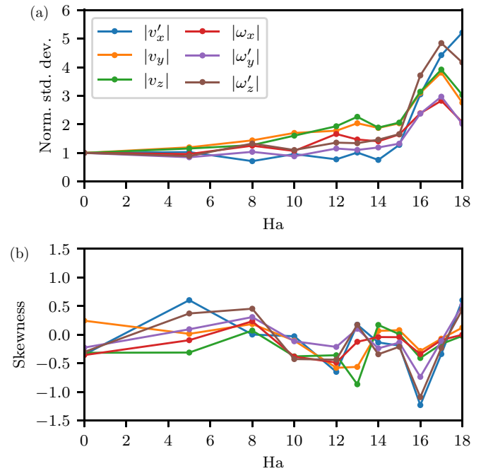
FIG. 14. Early warning statistics for the tipping point based on the statistics of various state variables (components of the velocity and vorticity perturbation). (a) Normalized standard deviation vs Ha ; (b) skewness vs Ha .
