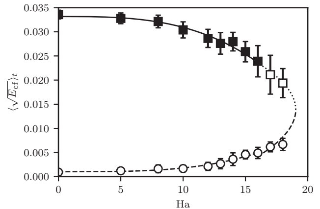
FIG. 13. Time-averaged square root of the cross-flow energy, \langle \sqrt{E_{cf}} \rangle_t , plotted vs Ha for the turbulent states (squares) and the edge states (circles). The error bars represent \pm one standard deviation. The axis \langle \sqrt{E_{cf}} \rangle_t = 0 corresponds to laminar flow. With reference to Fig. 12 and the definition of the edge state [8], stable and unstable/metastable states are plotted with full and open symbols, respectively. To estimate the value of Ha for the saddle-node bifurcation, a quadratic function is fitted to the data for Ha \geq 16 . The critical value is estimated as Ha_{sn} \approx 19 . Furthermore, power laws are fitted to the data as a guide to the eye. The fits are plotted using a solid line (stable states), a dotted line (metastable states), and a dashed line (unstable edge states).
