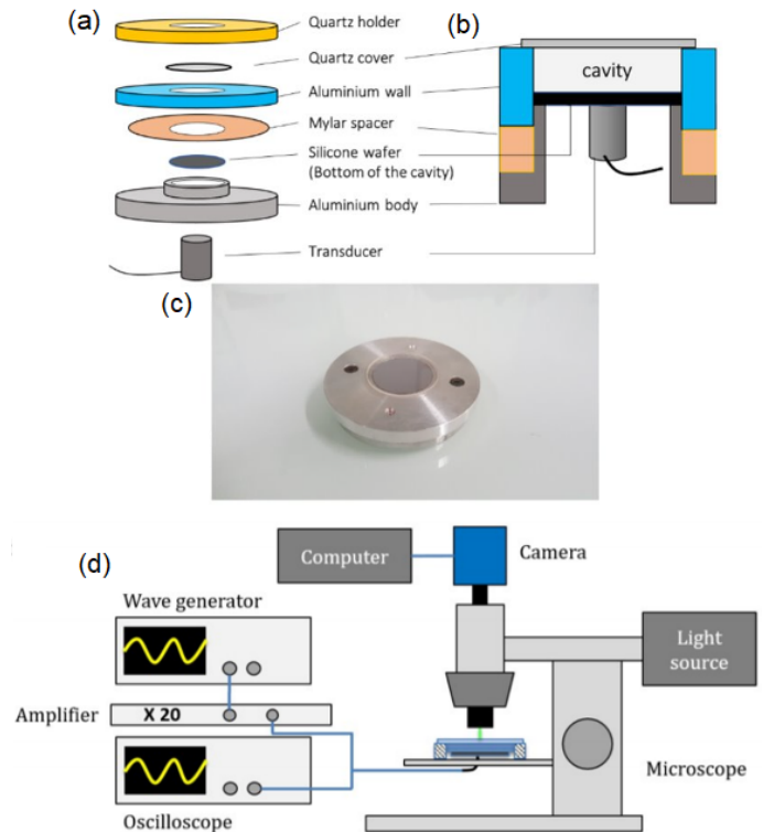
FIG. 2. Exploded view (a) and side view (b) of the cylindrical cavity used to study the motion of particles or cluster of particles induced by the ARF. Its diameter is 25 \text{ mm} a height h = 330 \mu\text{m} . c) Picture of the aluminum cavity. The drawings are not to scale. d) Sketch of the optic and acoustic setup. The cavity, coupled with the transducer, is placed on a motorized stage under a microscope. A signal generator is connected to the transducer to generate an acoustic wave, which is transmitted through the bottom of the cavity made of silicon. Observation and illumination are carried out through the quartz reflector at the top of the cavity (a). Axial and radial displacements of the particles can be monitored with a PCO™ Panda Bi camera plugged on the microscope [53].
