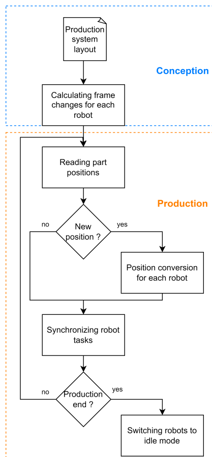
Figure 3: Environment layer flowchart
