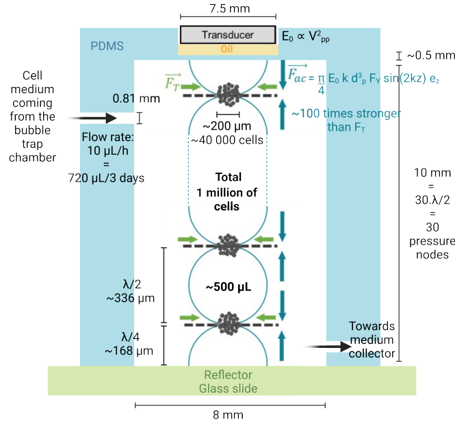
Figure 5. Schematic of the acoustofluidic well used in the present study to form and culture HepaRG spheroids over 6 days. The walls of the well are made of PDMS. An oil layer is used as a matching layer between the upper wall of the well and the transducer. The reflector facing the transducer is a glass slide. A constant flow rate is applied, allowing a total renewal of the medium after 3 days. The typical sizes of spheroids, as well as the internode distance obtained with a 2.2 MHz acoustic wave, are also displayed on the schematic.
