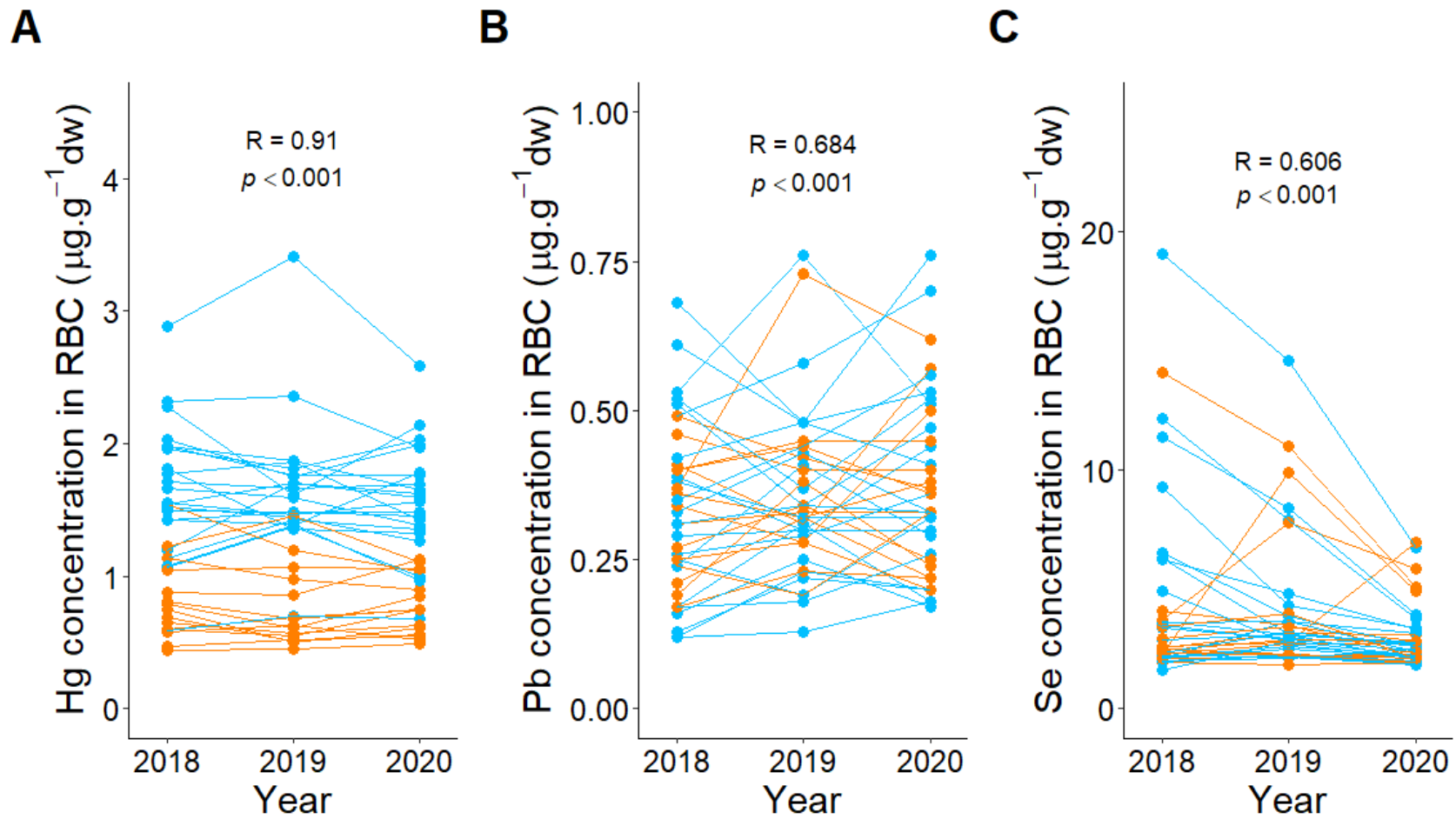
Figure 5. Hg (A), Pb (B), and Se (C) concentrations ( \mu\text{g.g}^{-1} dw) detected in red blood cells of E. orbicularis of two populations in the Camargue, France, during three years, n = 36 (blue: samples from Esquineau, orange: samples from Faïsses, R: coefficient of individual repeatability, p: significance)
