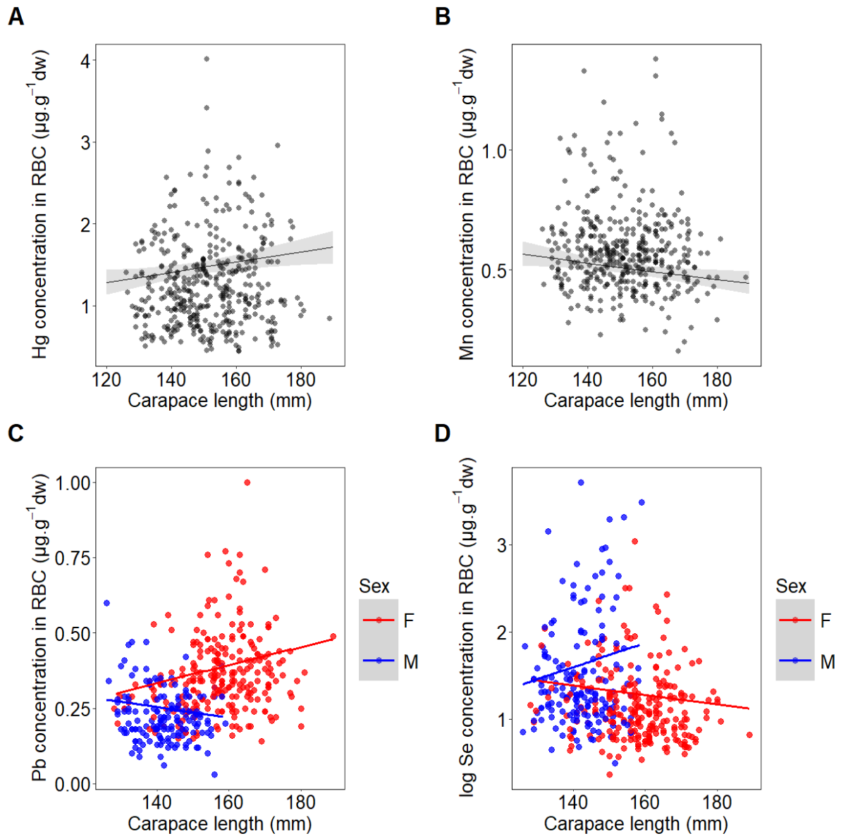
Figure 2. Relationship between Hg (A), Mn (B), Pb (C), and Se (D) concentrations ( \mu\text{g}\cdot\text{g}^{-1}\text{ dw} ) in red blood cells or carapace length (mm, A, B) or the carapace length in interaction with the sex (C, D) of the individuals sampled in the Camargue wetland (dots: data, lines: predictions of the mixed-effect models including (A) population, the sampling year and the DSL, R^2 conditional = 0.86, n = 410 ; (B) the sampling year and the DSL, R^2 conditional = 0.44, n_{\text{Female}} = 248 , n_{\text{Male}} = 162 ).
