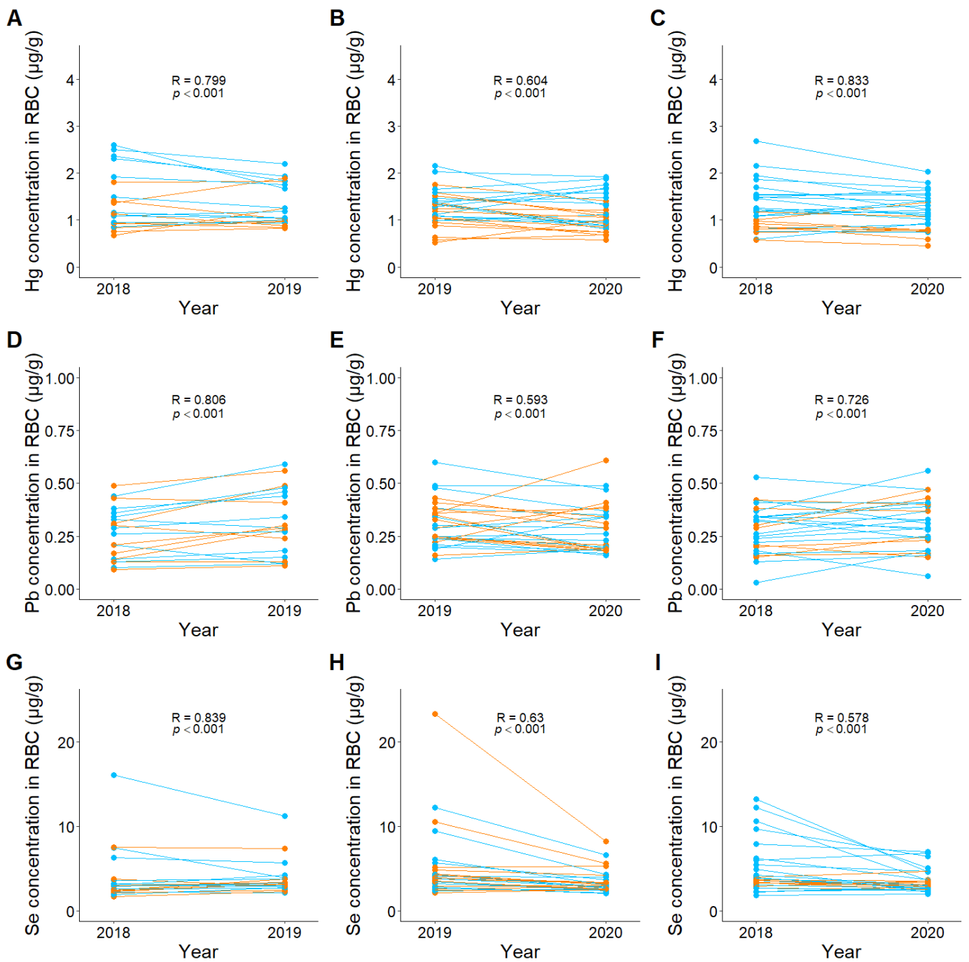
Figure S1. Hg (A, B, C), Pb (D, E, F), and Se (G, H, I) concentrations ( \mu\text{g}\cdot\text{g}^{-1} d.w.) detected in red blood cells of E. orbicularis of two populations in the Camargue, France, from 2018 to 2020, in individuals sampled for two years (blue: samples from Esquineau, orange: samples from Faïsses, R: coefficient of individual repeatability, p : significance)
