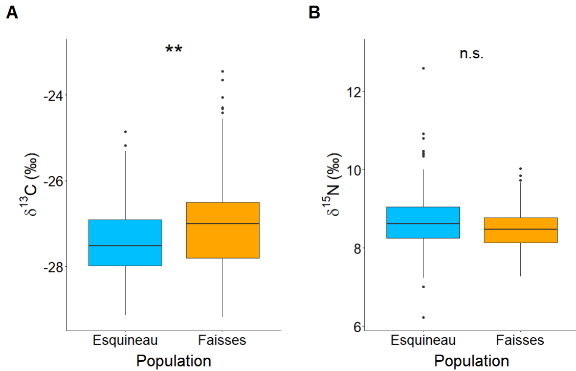
Figure 4. Variation in \delta^{13}\text{C} (A) and \delta^{15}\text{N} (B) in red blood cells of the individuals sampled in the Camargue wetland among the two populations: Esquineau and Faïsses, n = 409 (**: significance obtained from the LMM models)
