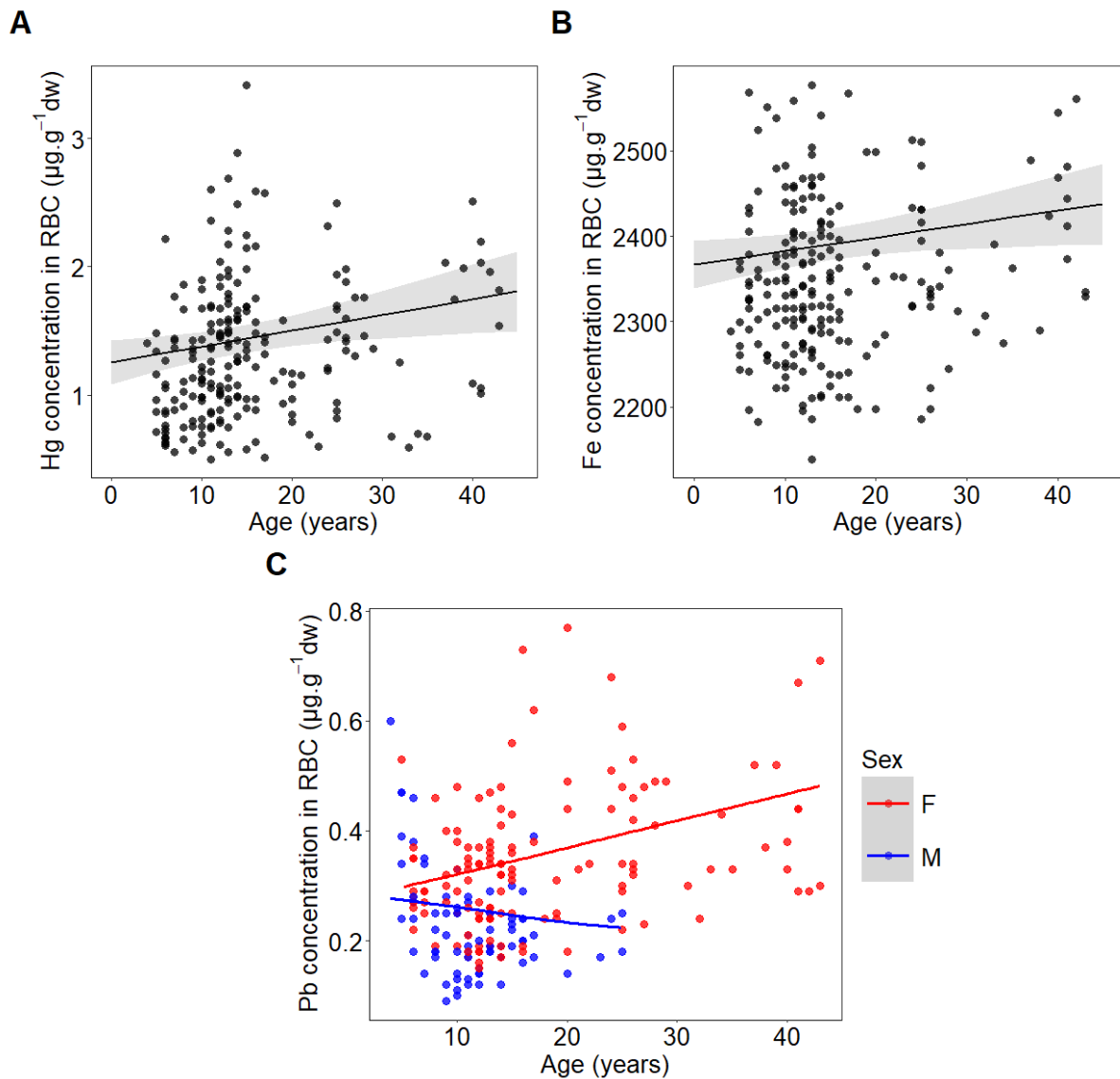
Figure 3. Relationship between Hg (A), Fe (B), and Pb (C) concentrations ( \mu\text{g}\cdot\text{g}^{-1} dw) in red blood cells and the age (year, A, B) and the age in interaction with the sex (C) of the individuals of known-age sampled in the Camargue wetland between 2018 and 2020 (dots: data, lines: predictions of the mixed-effect models including (A) population, the sampling year and the age, R^2 conditional = 0.83, n = 211 ; (B) the sampling year and the age, R^2 conditional = 0.45, n = 211 ; (C) the sampling year and the interaction of the sex and the age, R^2 conditional = 0.71, n_{\text{Female}} = 135 , n_{\text{Male}} = 76 ).
