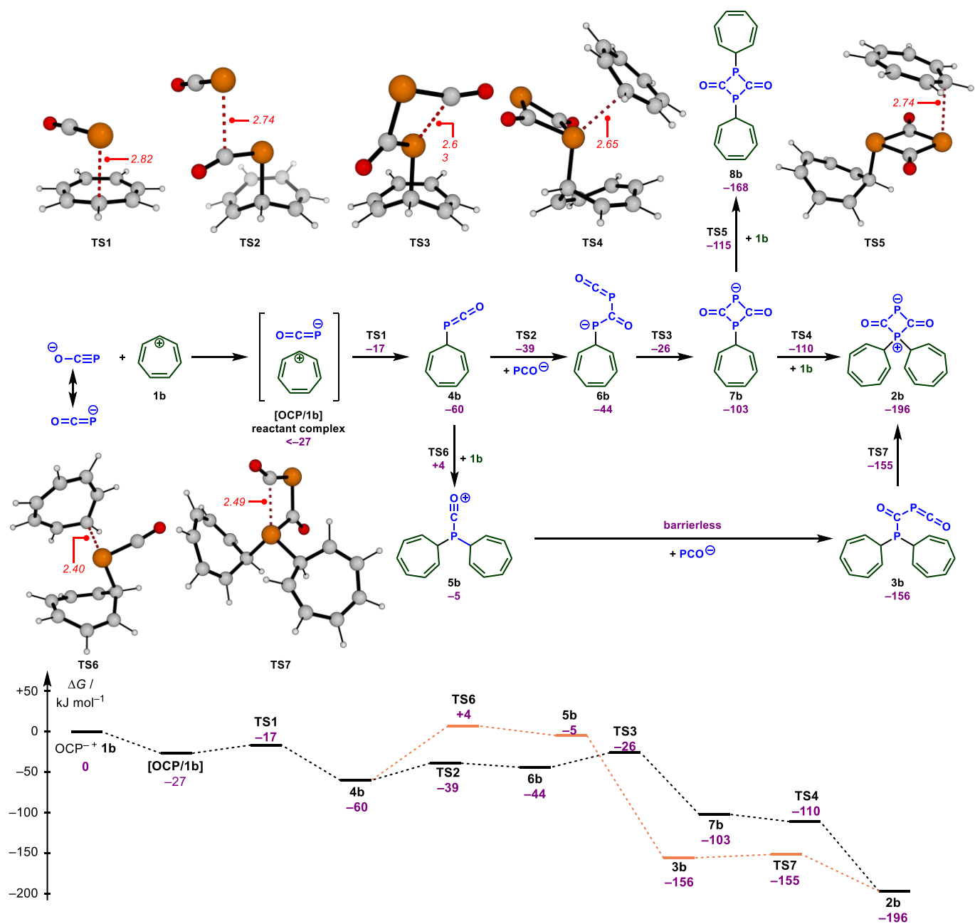
Scheme 4. Calculated reaction free energies (in kJ mol -1 ) and selected transition states (bond lengths in Å) for the proposed reaction mechanism for the formation of the zwitterion 2b and the phosphaketene 3b .
