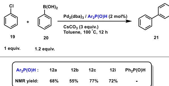
Scheme 10. Secondary phosphine oxide/ \text{Pd}_2(\text{dba})_3 catalysed the Suzuki cross-coupling reaction of 19 with 20 .
