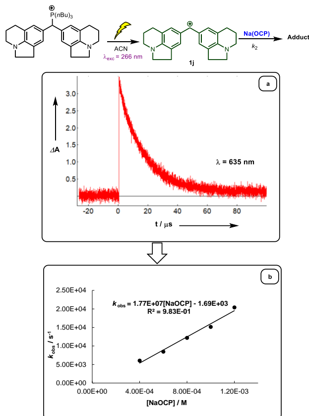
Figure 1. a) Decay of the absorbance of carbocation 1j obtained after irradiation of a 3.07 \times 10^{-5} \text{ mol L}^{-1} solution of the phosphonium salt 1j-P}(nBu) 3 in acetonitrile in the presence of \text{Na}(\text{OCP}) . b) Plot of the pseudo-first-order rate constants k_{\text{obs}} ( \text{s}^{-1} ) versus the concentration of \text{Na}(\text{OCP}) .
