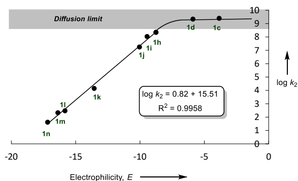
Figure 2. Plot of \log k_2 for the reactions of sodium phosphoethynolate Na(OCP) with reference electrophiles 1 , in acetonitrile at 20 °C versus their electrophilicity parameters E .
