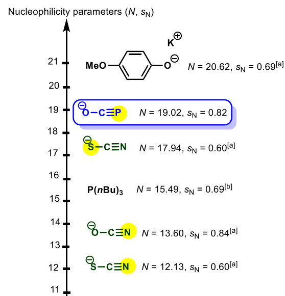
Figure 3. Embedding sodium phosphoethynolate in the Mayr nucleophilicity scale. [a] : solvent: acetonitrile. [b] : solvent: dichloromethane. 21, 22, 23, 24
