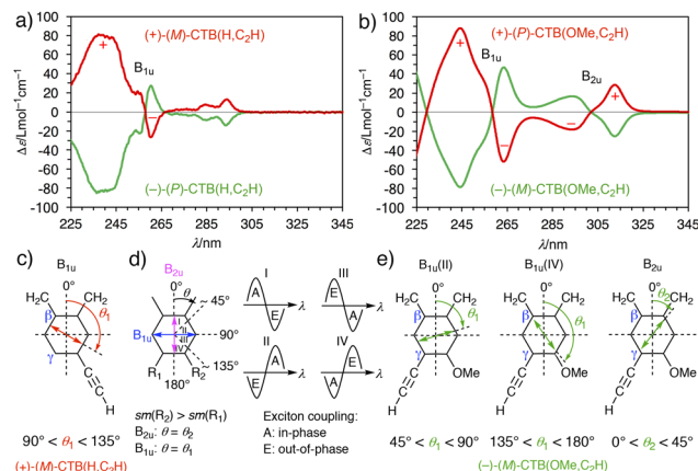
Fig. 4 Plots of the ECD spectra of (a) CTB(H,C 2 H) in CH 2 Cl 2 and (b) CTB(OMe,C 2 H) in CH 3 CN between 225 and 345 nm, which covers the regions of the B 1u and B 2u transitions. The ECD spectrum of CTB(OMe,C 2 H) in the full range is shown in Fig. S64b.† The spectra of the first eluted enantiomers are in green, those of the second eluted enantiomers are in red. In (c) and (e) are represented the directions of polarization (angle \theta_1 ) of the B 1u transitions of (M)-CTB(H,C 2 H) and (M)-CTB(OMe,C 2 H). Two are possible in the case of the latter compounds. They are discussed in the text. In (e) is also represented the direction of polarization (angle \theta_2 ) of the B 2u transition of (M)-CTB(OMe,C 2 H). It is lacking for the B 2u transition of (M)-CTB(H,C 2 H), because this transition does not show an exciton couplet. (d) The orientations of the dipole moments of the transitions B 1u and B 2u of benzene are shown in blue and pink, respectively. The expected shapes of the exciton couplets of the B 1u and B 2u transitions as a function of the location of the direction of polarization of the transition dipole in quadrants I ( 0^\circ < \theta < 45^\circ ), II ( 45^\circ < \theta < 90^\circ ), III ( 90^\circ < \theta < 135^\circ ), and IV ( 135^\circ < \theta < 180^\circ ) are also shown. See ref. 43 and 46 for details.
