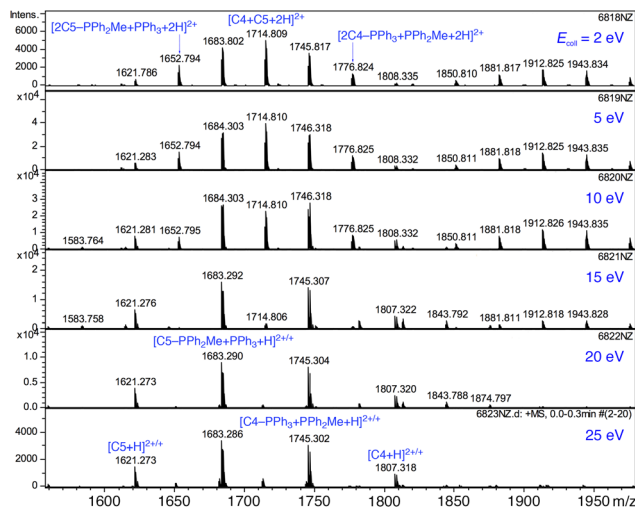
Fig. 6 Evolution of the ESI-MS spectra of a 1 : 1 mixture of 10^{-4} M solutions of complexes C4 and C5 in \text{CHCl}_3/\text{i-PrOH}/\text{HCO}_2\text{H} 50 : 49.5 : 0.5.
