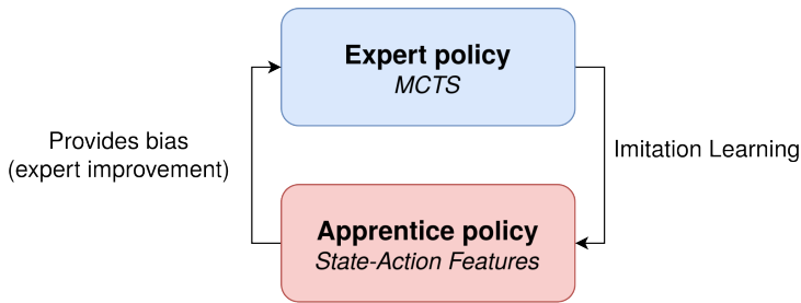
Figure 2.4: Feedback loop of the expert iteration framework. The apprentice learns from the expert by trying to mimick its policy, while the expert itself is biased by the apprentice as it learns. In our specific framework, the expert policy is obtained from an MCTS algorithm, itself biased by learnt state-action features.
