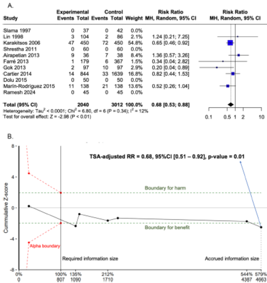
Fig. 3 A Forest plot comparing the incidence of central venous catheter infections (composite outcome) between ultrasound-guided versus anatomical landmark technique. B Trial Sequential Analysis
