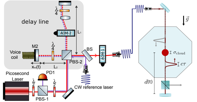
FIG. 1. Overview of our experimental setup. The picosecond laser (red line) is split in two on the polarizing beam splitter PBS-2. One part is sent directly to the vacuum chamber and is retro-reflected by a mirror placed below the chamber. The other part passes through a delay line. The mirror M2 of the delay line is moved using a voice coil actuator. A cw reference laser, with a known wavelength (in purple), is used to measure the position of M2 using a heterodyne detection scheme.
