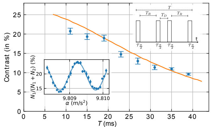
FIG. 4. Contrast of the central fringe as a function of the total interrogation time with \tau = 1.47 ps, a \pi -pulse duration of 0.6 ms and T_D of 3 ms. Experimental data are shown in blue. The Monte-Carlo simulation is shown in the orange full line. Typical fringes are shown in the bottom inset for T = 39 ms. The contrast is deduced from a fit of the fringes (blue line). The upper insert shows the interferometer sequence
