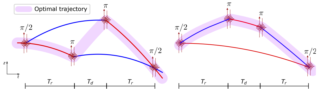
FIG. 5. Illustration of the atomic wave packet trajectories for a \pi/2 - \pi - \pi - \pi/2 pulse sequence. The vertical axis represents the atoms' vertical position and the horizontal axis is time. The blue and red colors distinguish the internal states. The pink shaded lines show the trajectory of the overlap zone controlled via the M2 mirror.
