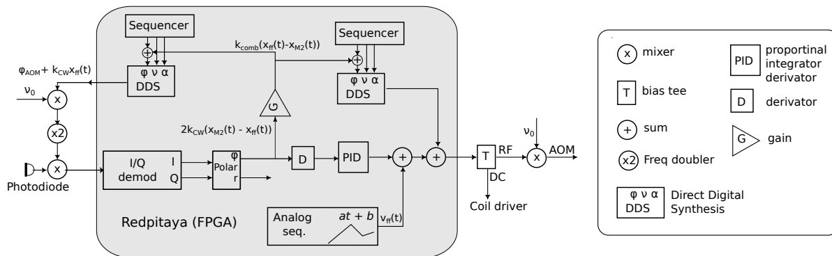
FIG. 2. Schematic of the control system implemented using a redpitaya board. To accommodate for the relatively low bandwidth of the board (50 MHz), we use frequency mixers to shift the frequencies from the digital to analog converter to the AOM and from the photodiodes to the analog to digital converter. The command of the coil driver is digitally added to the rf in the FPGA and then extracted using a bias T, to accommodate the limited number of outputs of the board.
